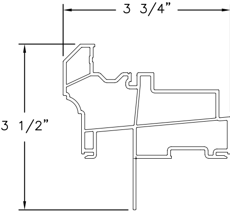
HEAD FRAME, FIN (10008687) VINYL PVC
