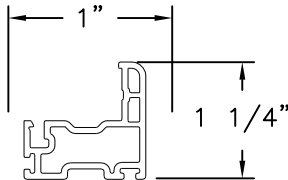
STILE (10008842) VINYL PVC
