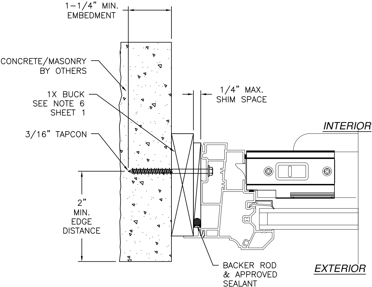
JAMB INSTALLATION DETAIL CONCRETE/MASONRY W/1X BUCK INSTALLATION
