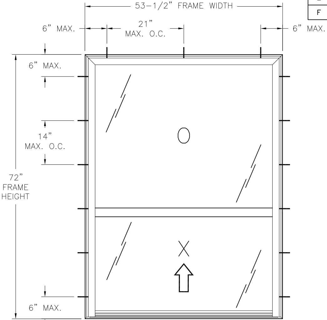
SERIES 1441 VINYL SINGLE HUNG ORIEL WINDOW EXTERIOR VIEW
