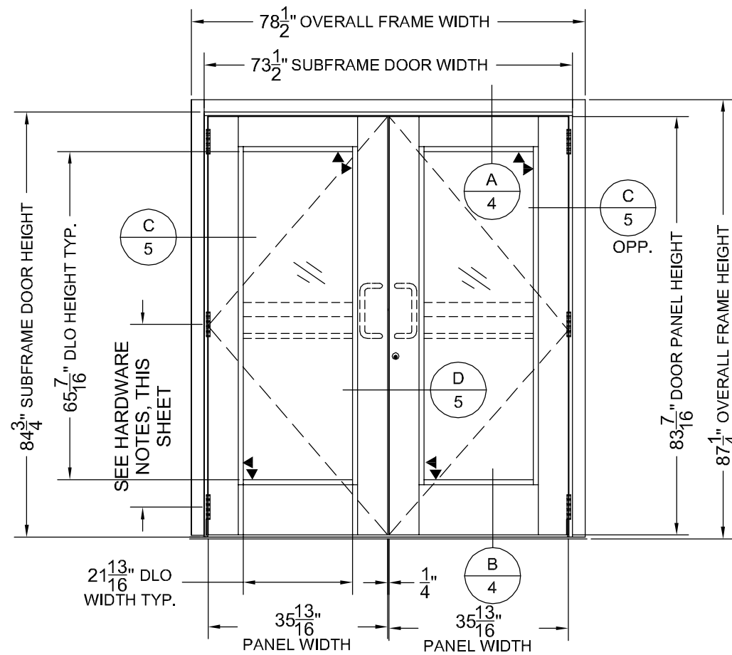
ELEVATION C
