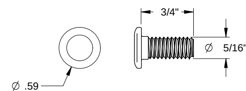
TRACK BOLT
