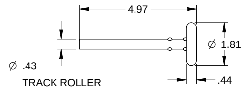
TRACK ROLLER
