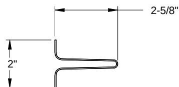
U-BAR 18 GA. (.049" MIN) GALVANIZED 80 KSI MINIMUM TENSILE
