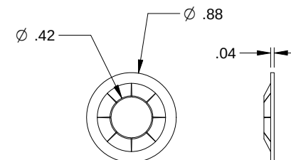
RETAINING NUT
