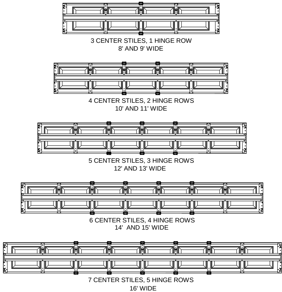
CENTER STILE / HINGE ROW LAYOUT NON-GLAZED SECTIONS SHOWN INTERIOR VIEW
