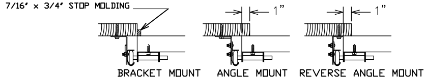
JAMB OVERLAP DETAIL
