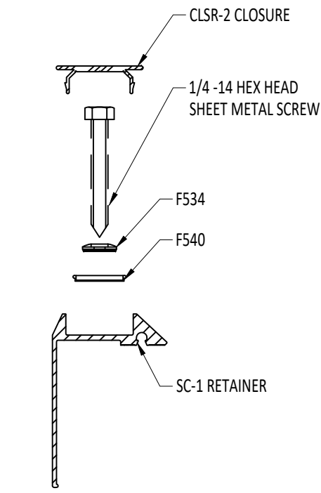
SNAP LOCK DETAIL
