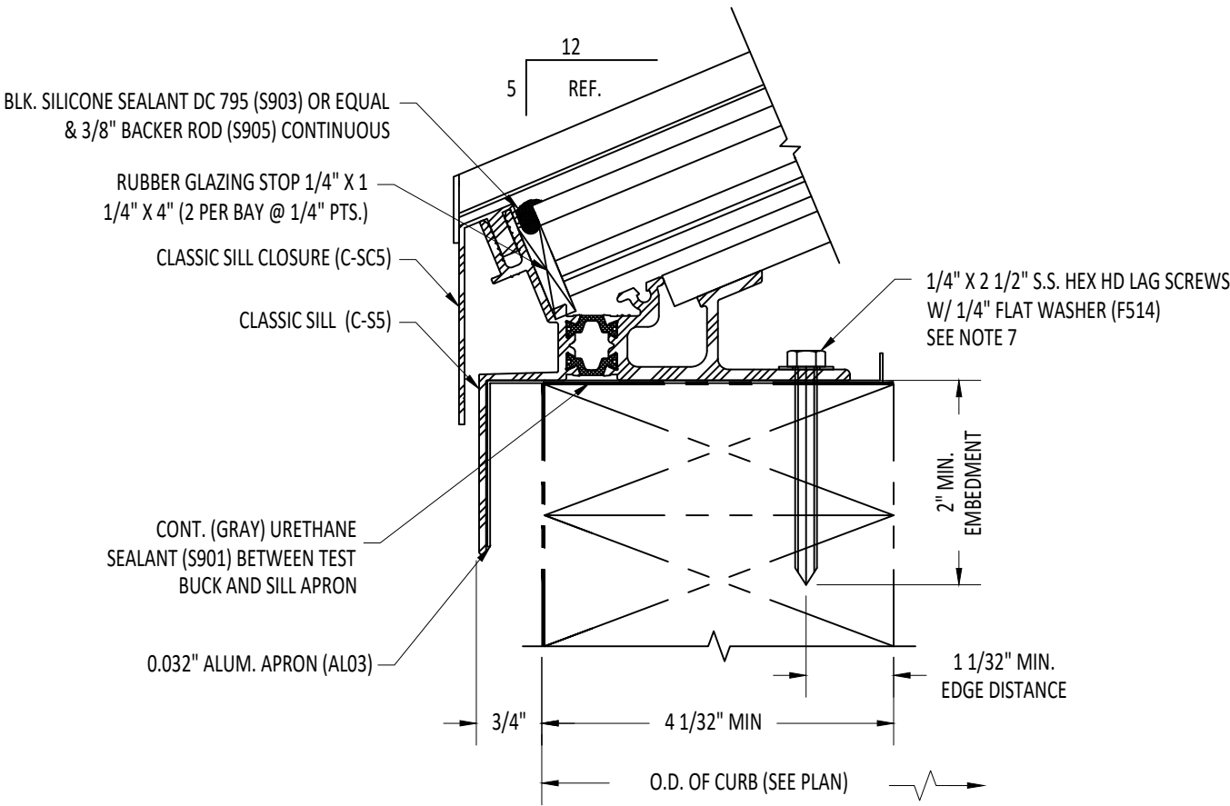
1/2 INSTALLATION DETAIL
