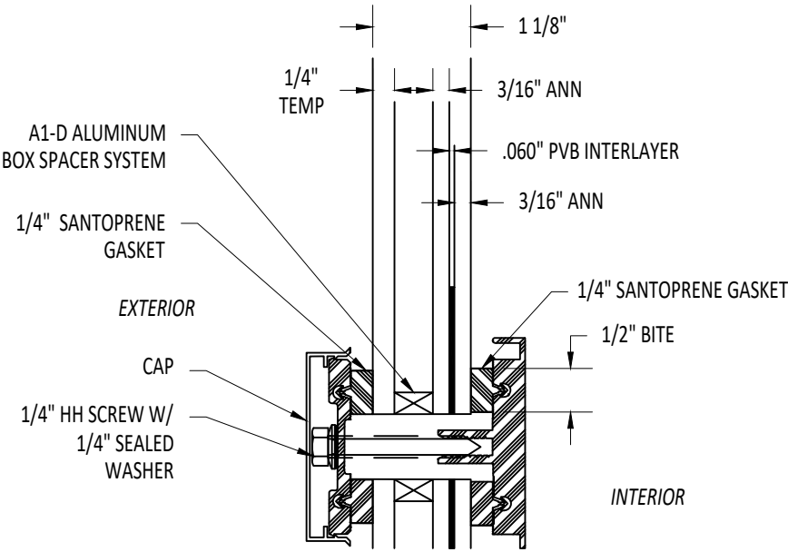
GLAZING DETAIL
