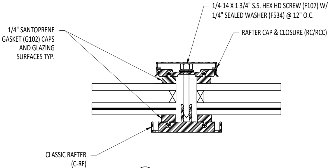
3/2 RAFTER INSTALLATION DETAIL
