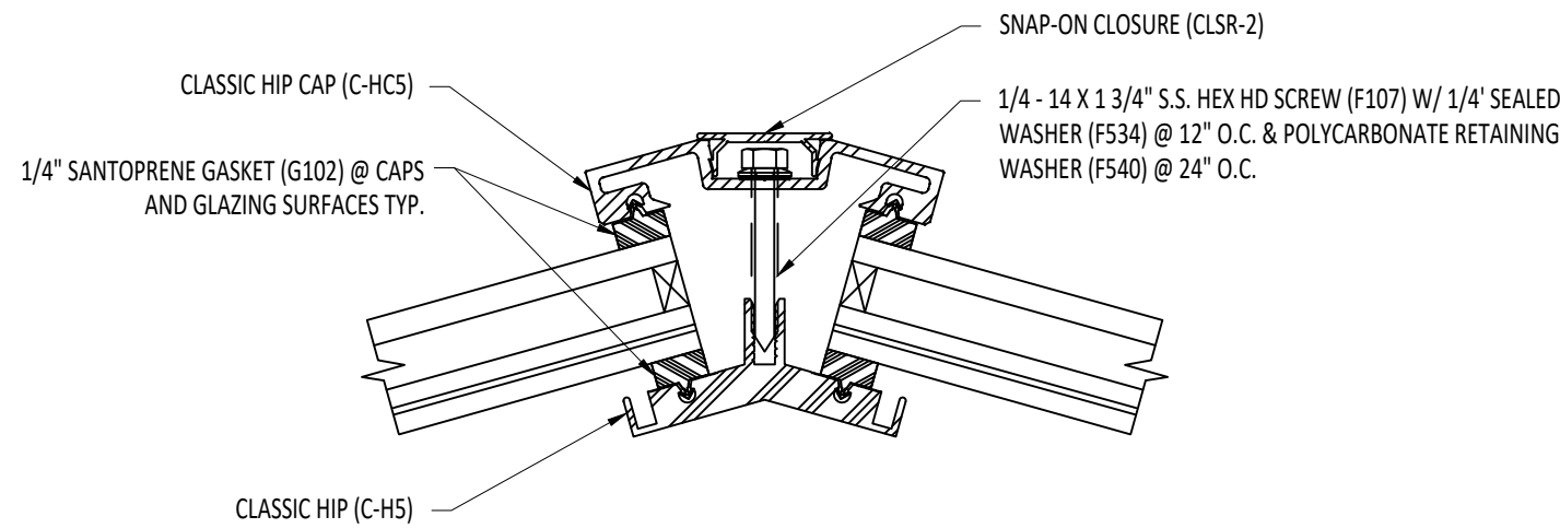
2/2 HIP INSTALLATION DETAIL
