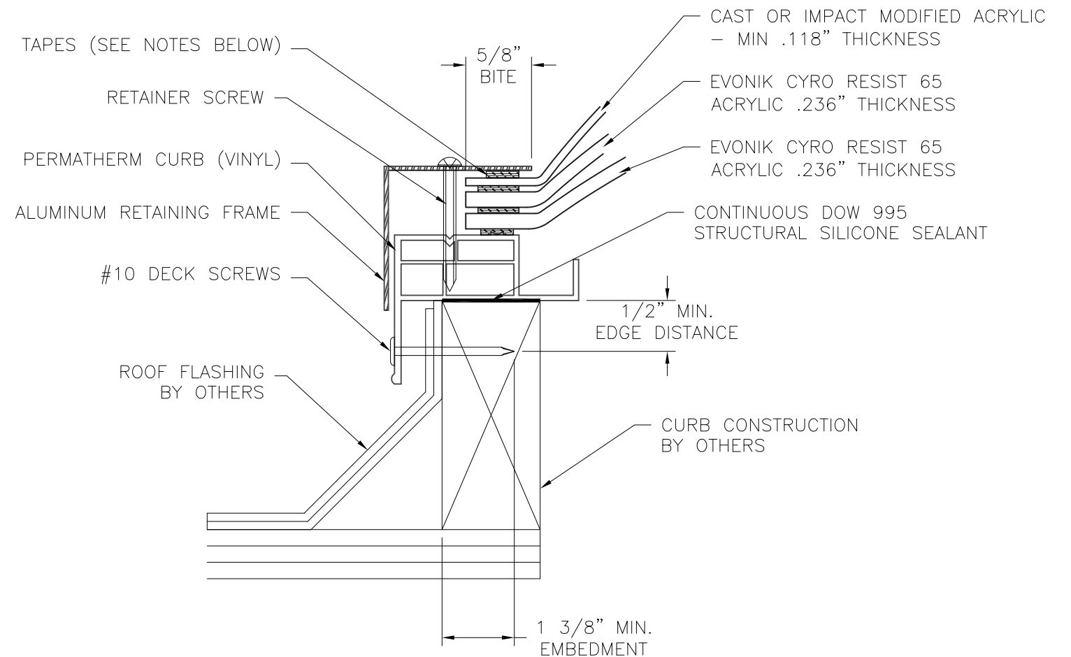
INSTALLATION DETAIL (WITH TRIPLE GLAZING)
