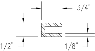
ALUM. CHANNEL SPACER (6063-T5)
