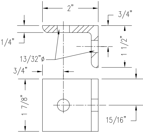
ALUM. RAFTER CLIP @ CTR RAFTERS (6061-T6)
