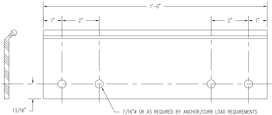
BASE PLATE DETAIL (BP-1) SCALE: 6" = 1'-0'
