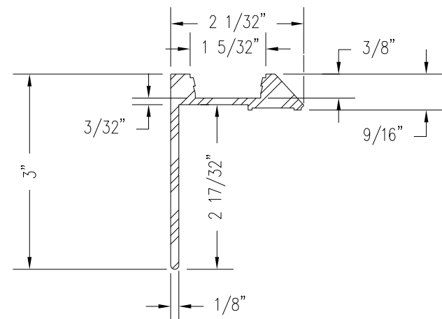
SILL PERIMETER TAPE CAP EXTRUSION (H-PC)
