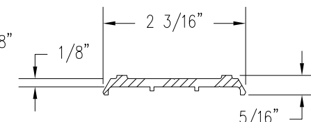
VE MULLION CAP EXTRUSION (H-MC)
