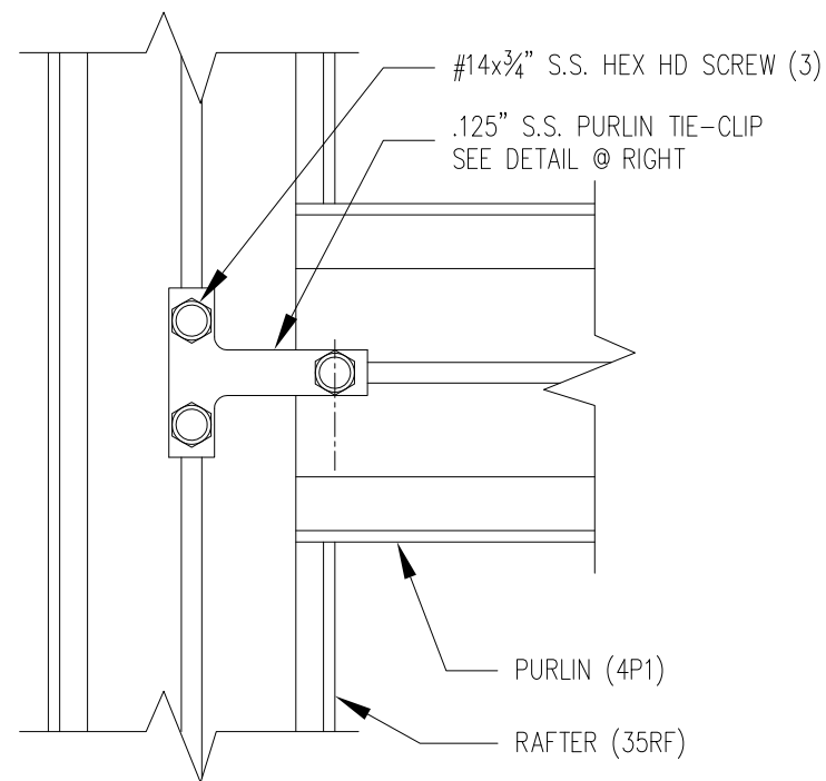
END RAFTER TO PURLIN CONNECTION
