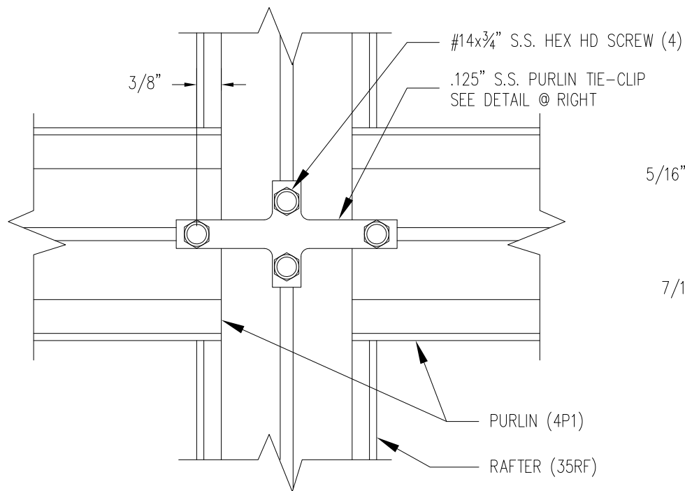
RAFTER TO PURLIN CONNECTION
