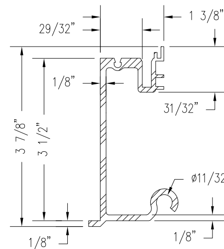
RIDGE/HIP EXTRUSION (35H-1F)
