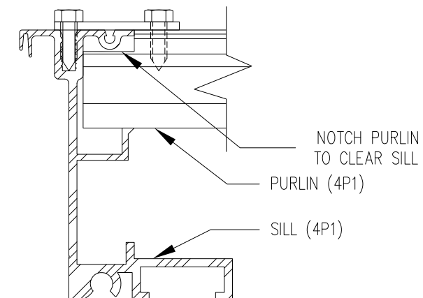
PURLIN TIE-CLIP (SILL & END RAFTER TO PURLIN) (A304 STAINLESS STEEL)
