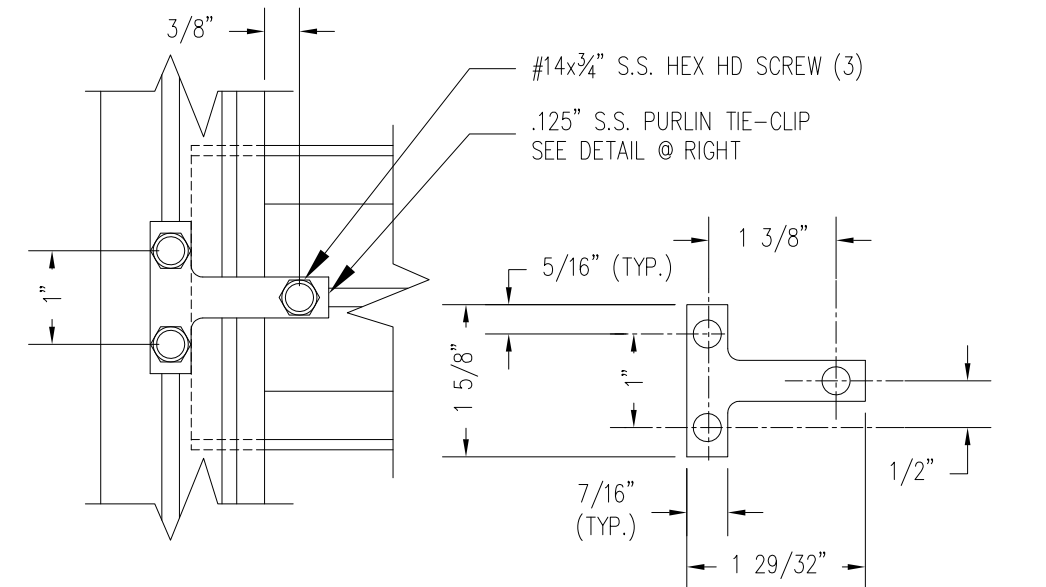
PURLIN TIE-CLIP (SILL & END RAFTER TO PURLIN) (A304 STAINLESS STEEL)
