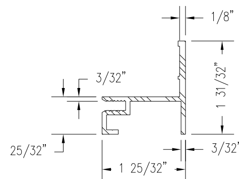
VE SASH EXTRUSION (H-HS)
