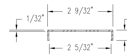
VE MULLION CLOSURE EXTRUSION (H-MCC)
