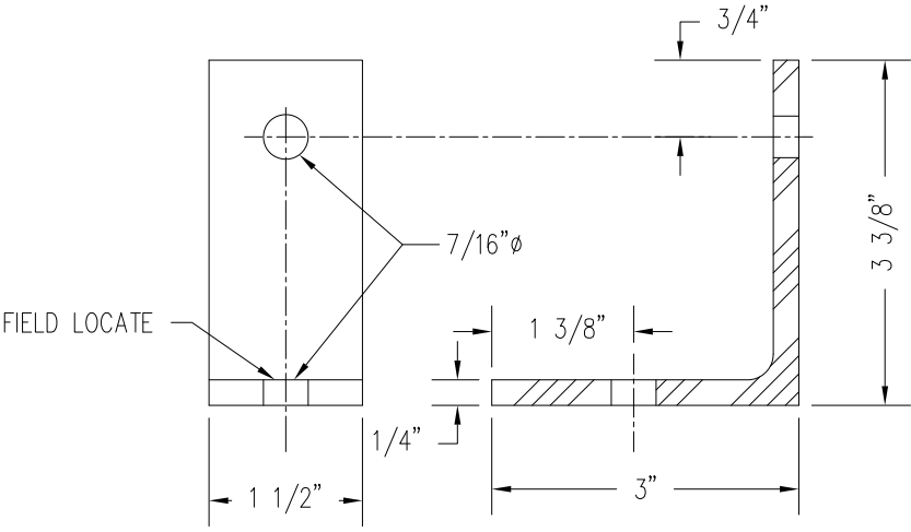
ALUM. RAFTER SUPPORT ANGLE @ SILL END (6061-T6) DIMS. MAY VARY W/ UNIT PITCH
