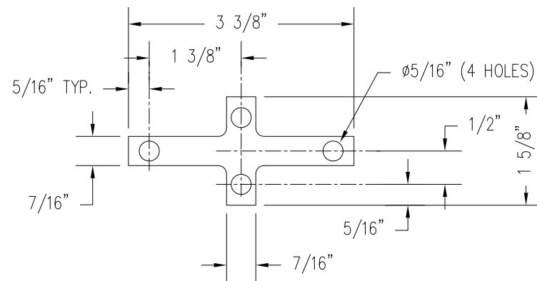
PURLIN TIE-CLIP (RAFTER TO PURLIN) (A304 STAINLESS STEEL)
