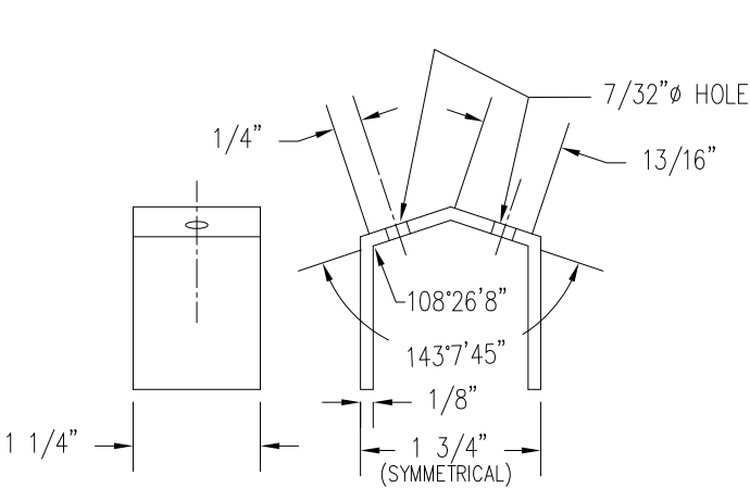
VE MULLION ALUM. TOP CLIP (VARIES W/ UNIT PITCH)
