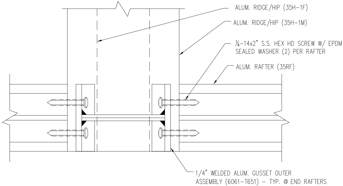
SECTION C-C END RAFTER TO RIDGE/HIP GUSSET CONNECTION DETAIL
