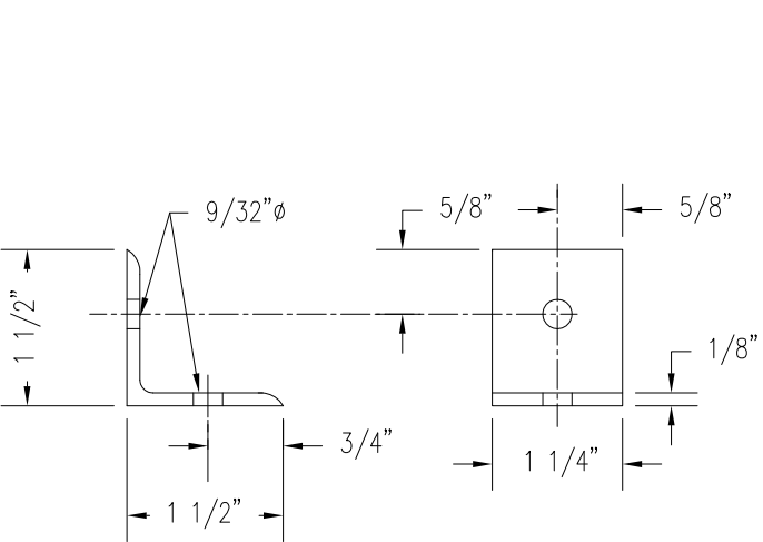
VE MULLION ALUM. BOTTOM SUPPORT ANGLE
