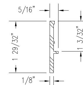
SASH CAP EXTRUSION (H-SC)
