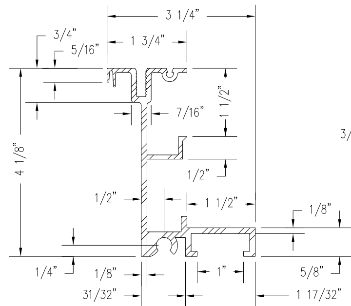
SILL EXTRUSION (35S)
