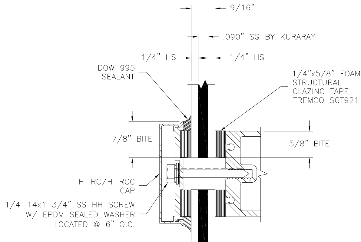
GLAZING A
