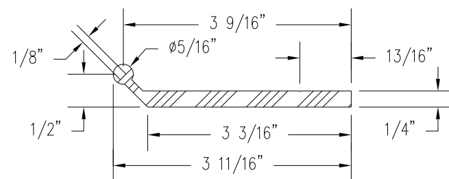
BASE PLATE EXTRUSION (BP-1)
