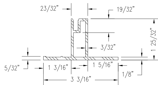
VE RAKE SASH EXTRUSION (H-RS)
