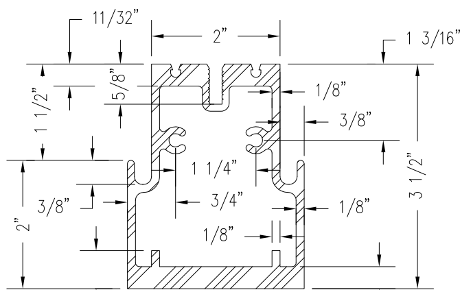
SILL EXTRUSION (35S)
