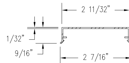
CLOSURE EXTRUSION (H-RCC)
