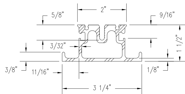
PURLIN EXTRUSION (4P1)
