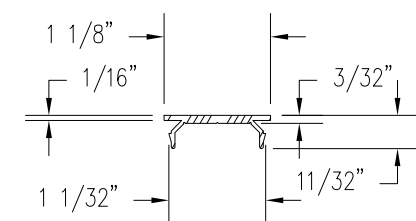
SILL CLOSURE CAP EXTRUSION
