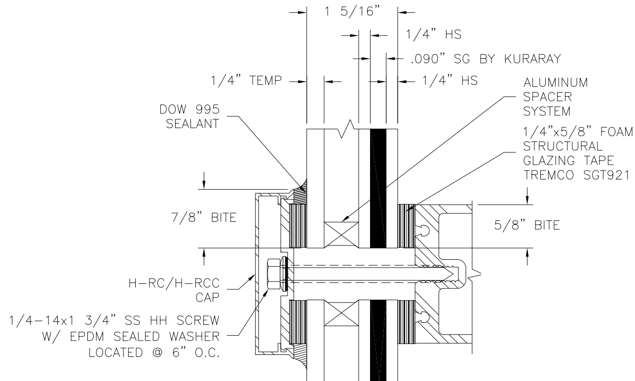
GLAZING B
