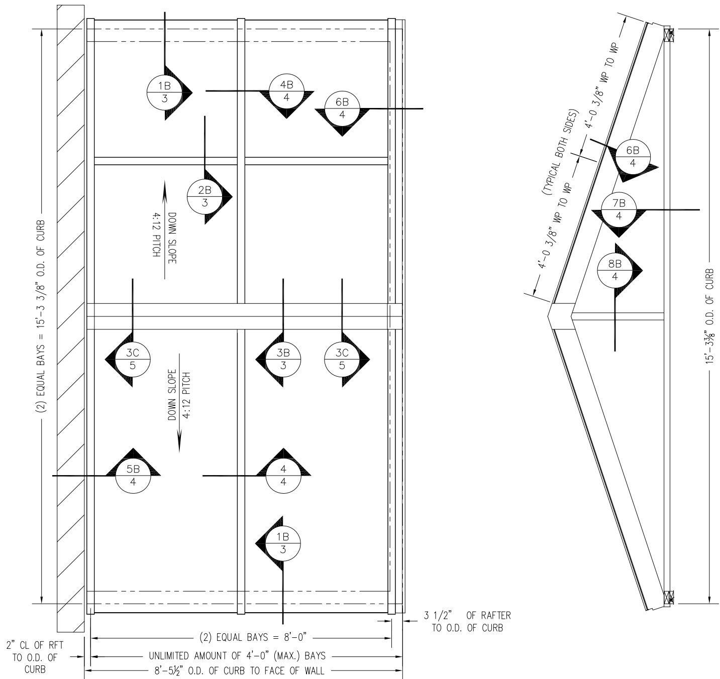
PINNACLE - HU SKYLIGHT PLAN VIEW
