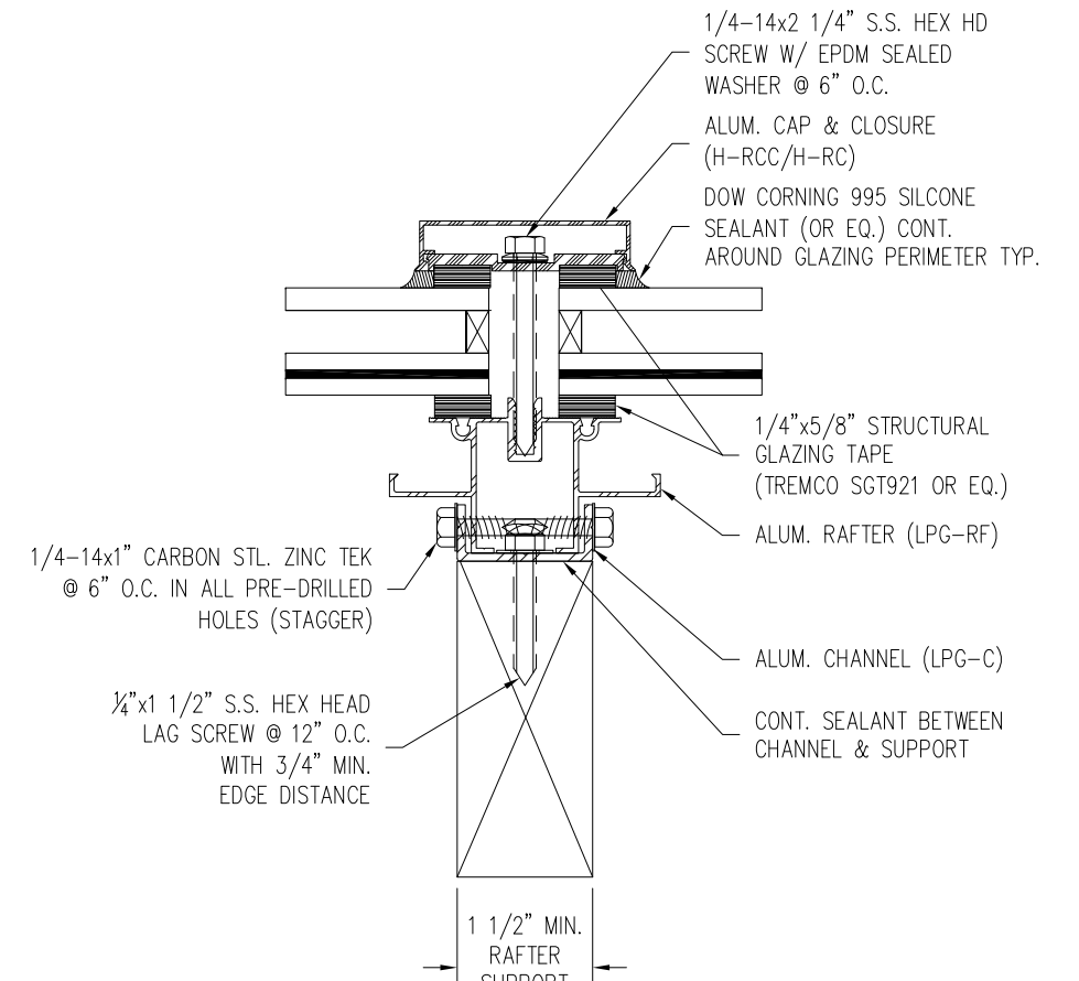
RAFTER DETAIL
