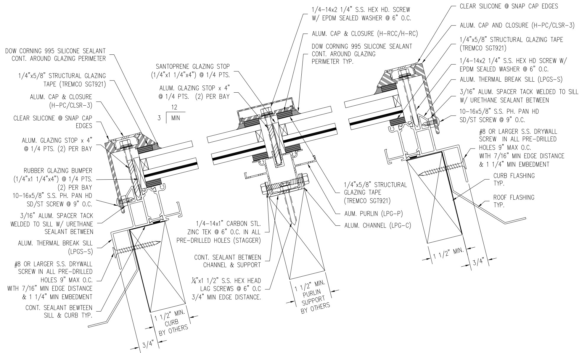
VERTICAL CROSS SECTION INSTALLATION DETAIL
