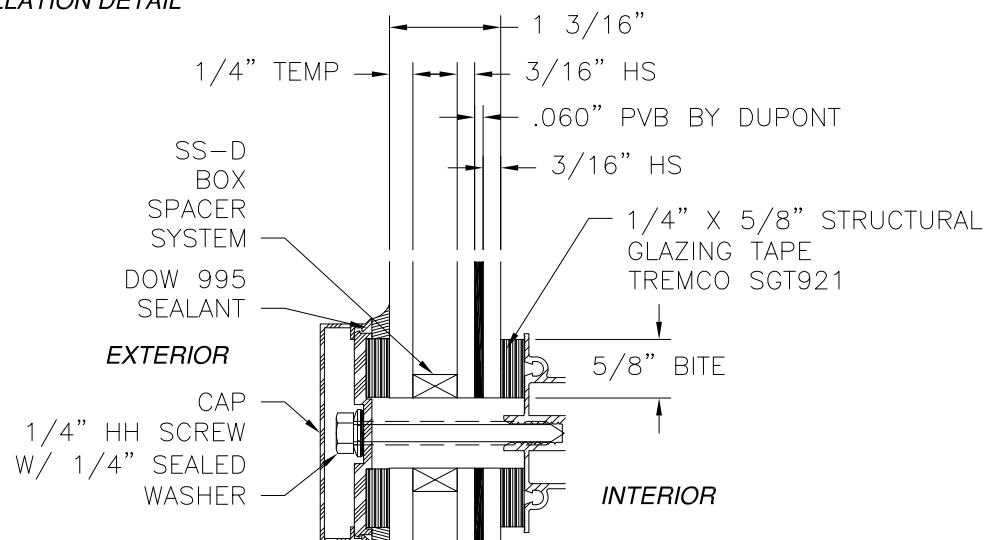
GLAZING DETAIL
