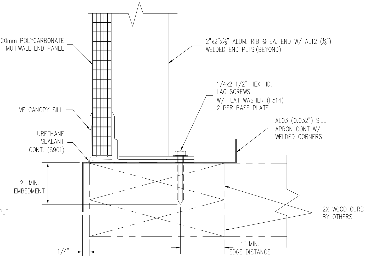
VERTICAL SILL DETAIL
