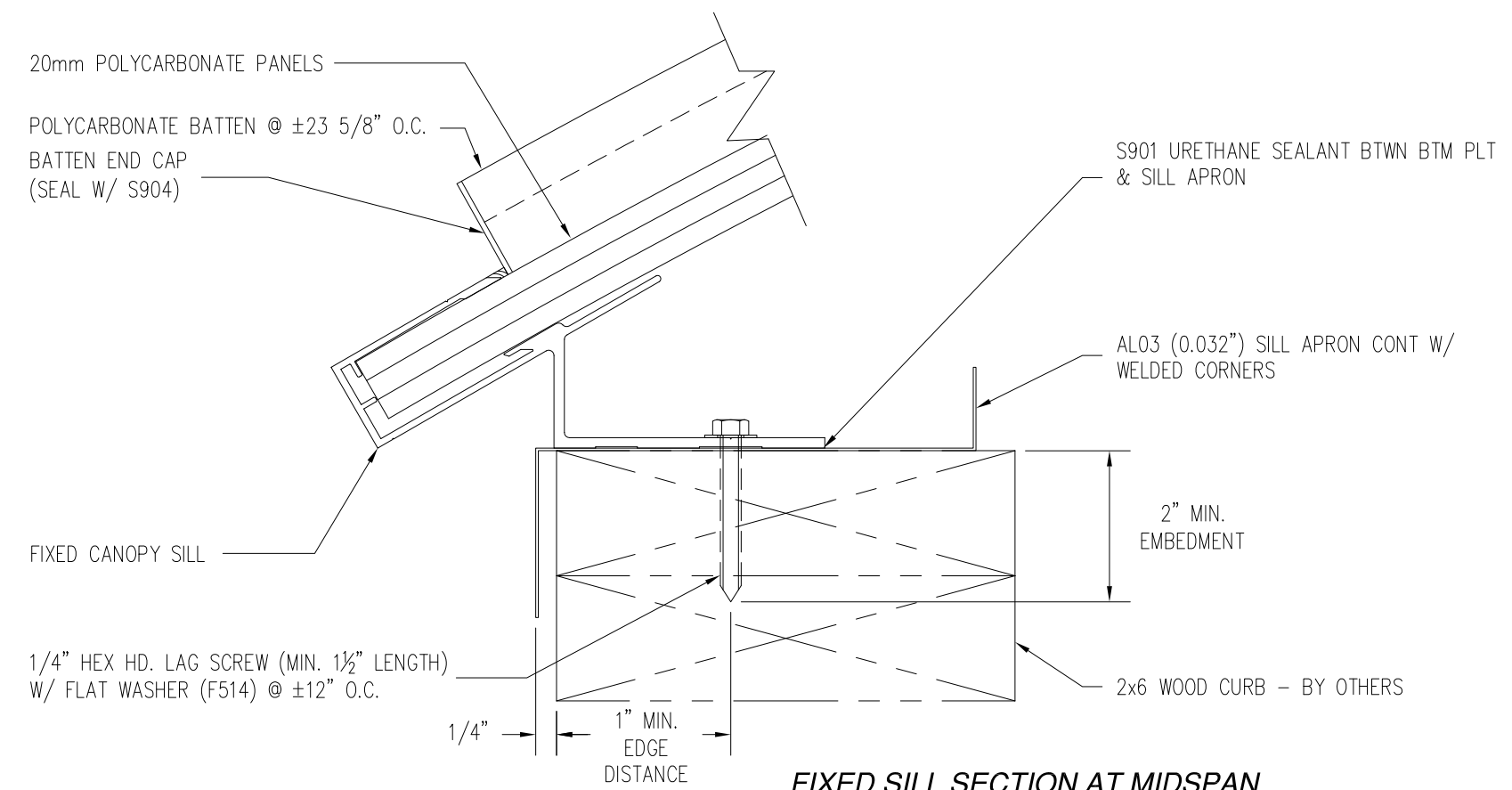
FIXED SILL SECTION AT MIDSPAN
