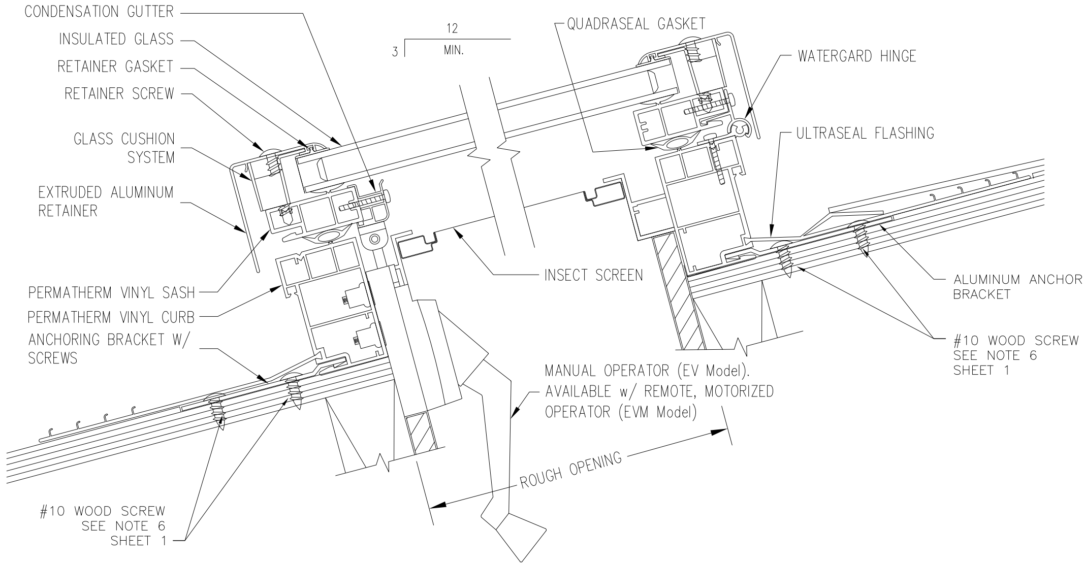
FLASHING LEGS AT JAMBS INSTALLATION DETAIL
