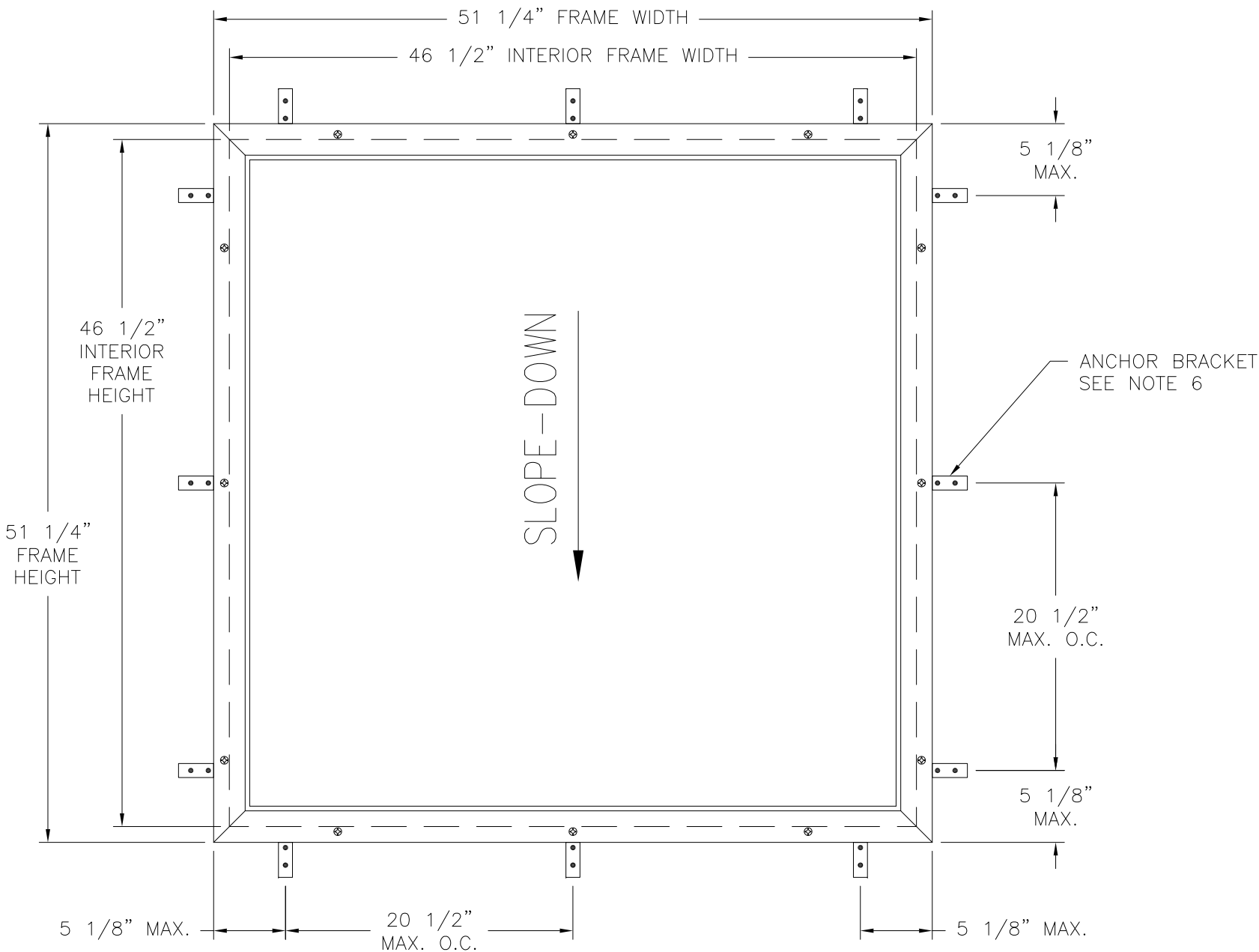
EV SKYLIGHT (47X47) PLAN VIEW FLASHING NOT SHOWN FOR CLARITY
