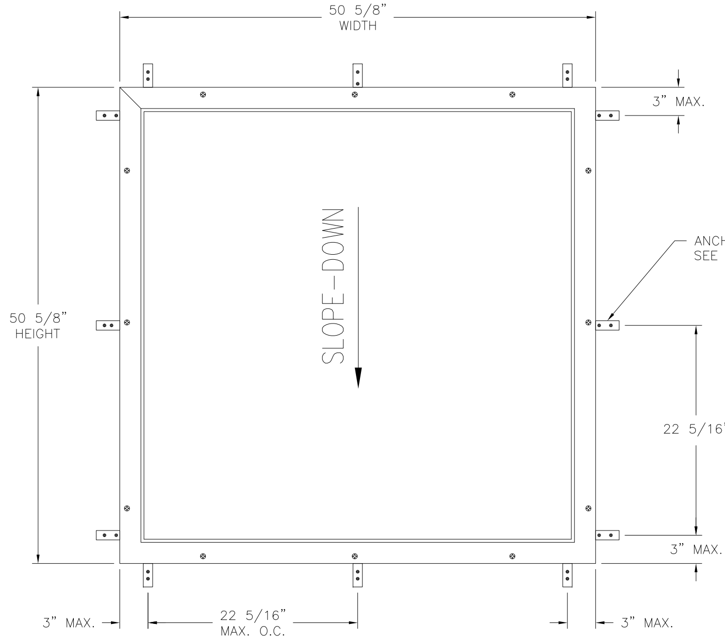
EFHR 4646 SKYLIGHT PLAN VIEW FLASHING NOT SHOWN FOR CLARITY
