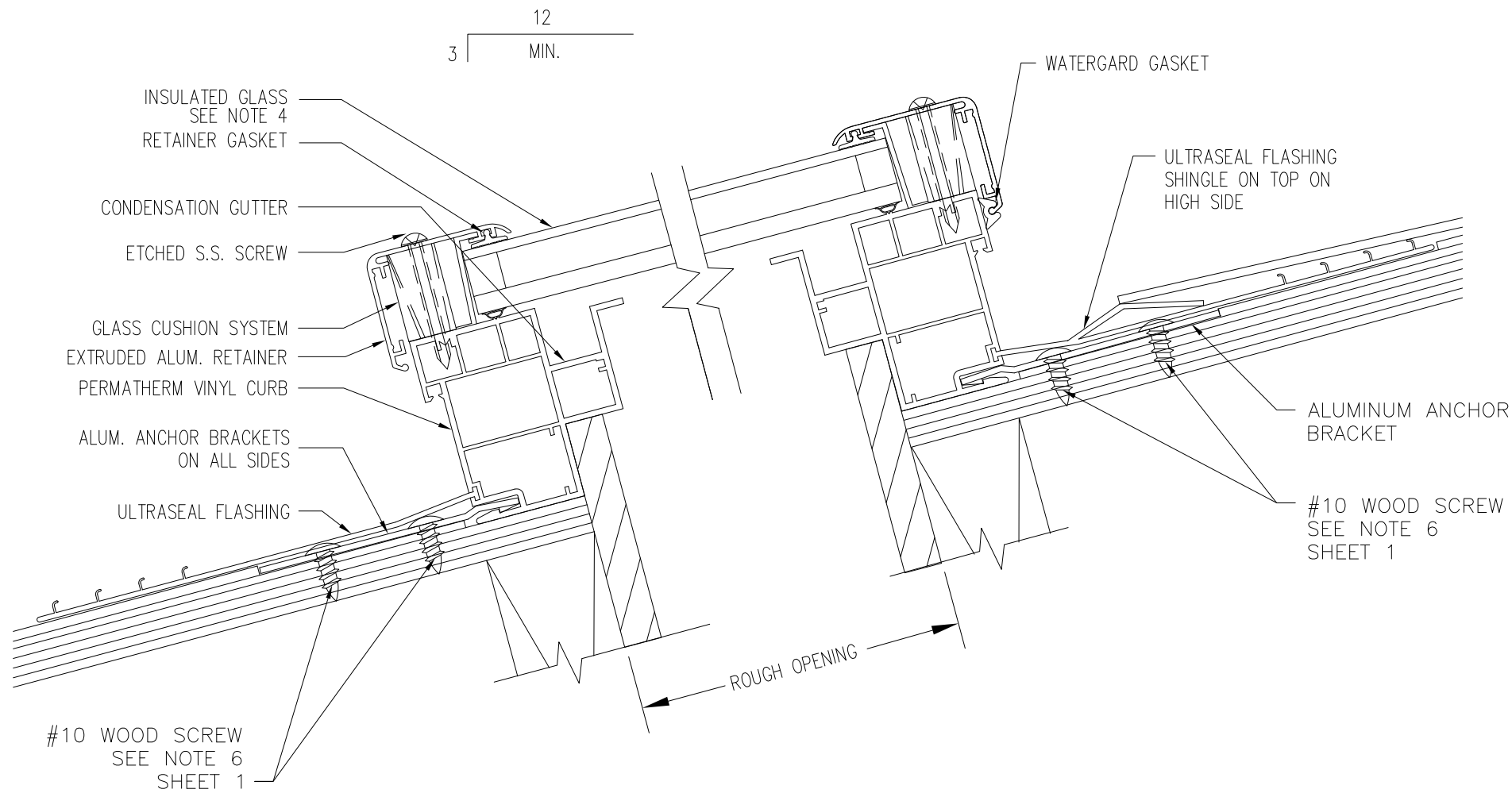
INSTALLATION DETAIL
