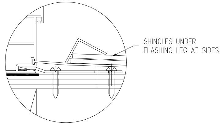
FLASHING LEGS AT JAMBS INSTALLATION DETAIL
