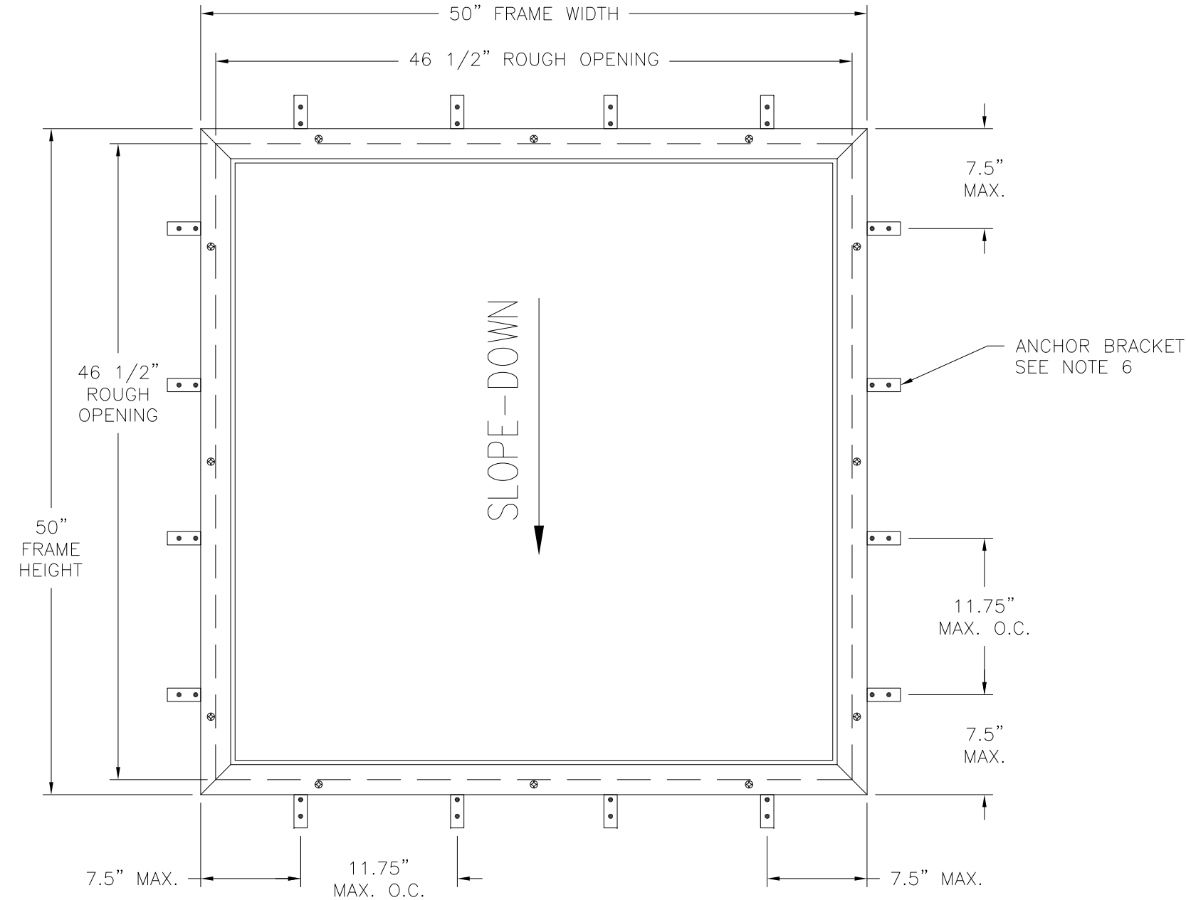
EF SKYLIGHT (47X47) PLAN VIEW FLASHING NOT SHOWN FOR CLARITY
