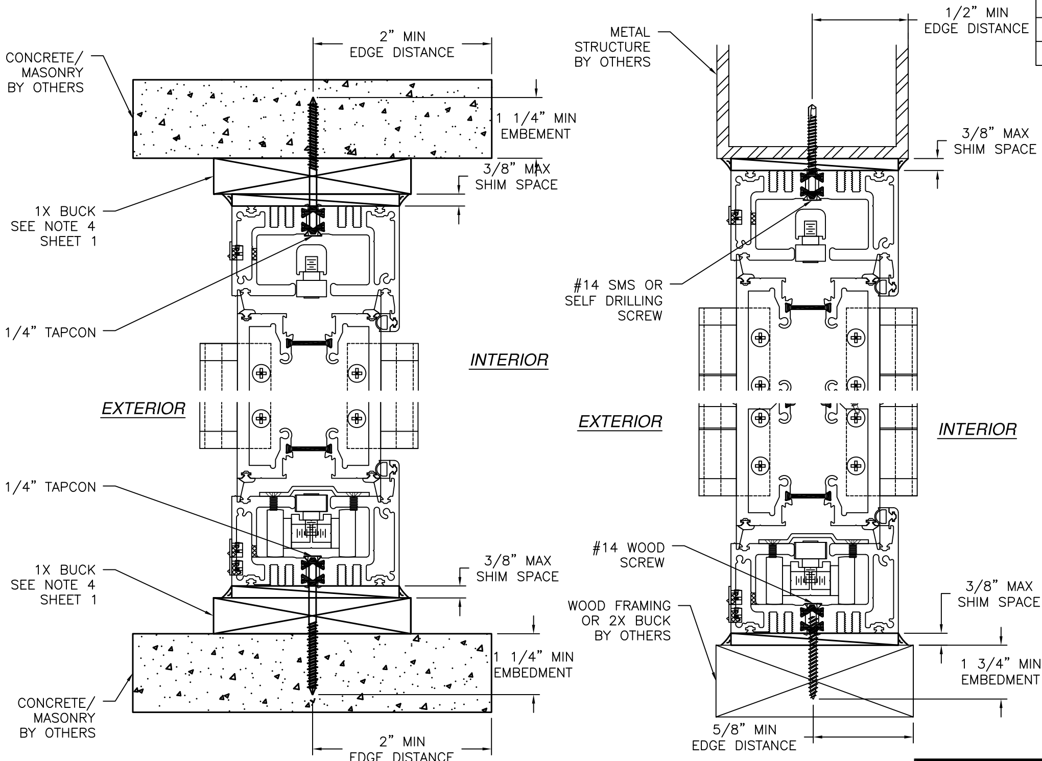
VERTICAL CROSS SECTION CONCRETE/MASONRY INSTALLATION OUTSWING SHOWN, INSWING SIMILAR
