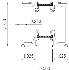
REGULAR THERMAL FRAME
