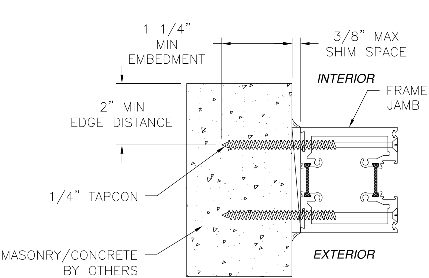
JAMB INSTALLATION DETAIL MASONRY/CONCRETE
