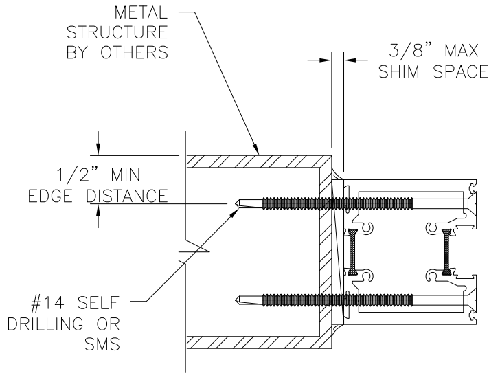
JAMB INSTALLATION DETAIL METAL STRUCTURE
