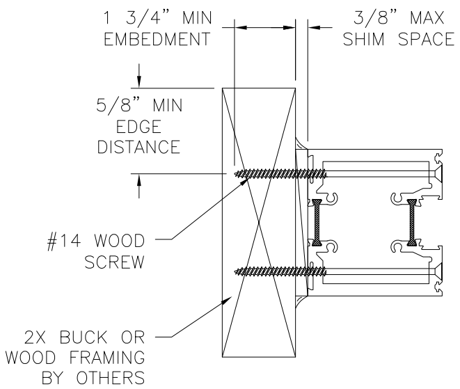
JAMB INSTALLATION DETAIL 2X BUCK OR WOOD FRAMING
