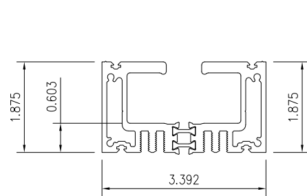
FLUSH SILL
