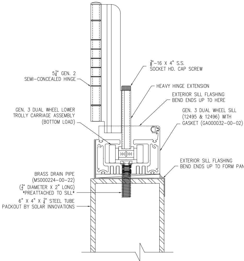
DRAIN PIPE AND HINGE EXTENSION DETAIL
