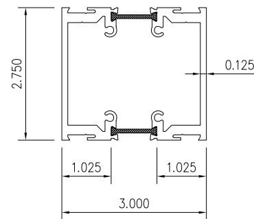
HORIZONTAL MULLION
