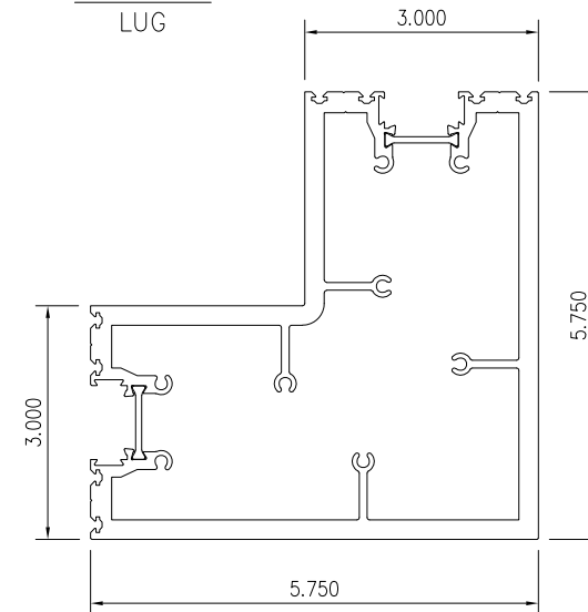
KNUCKLE JAMB
