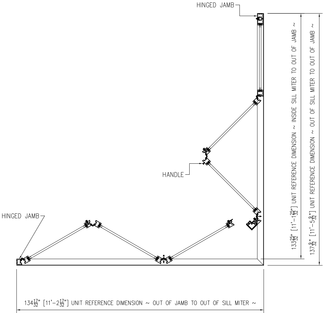
SERIES SI3000 FGW 3.5X9.5 PANEL 90° CORNER NO-POST - STANDARD SILL
