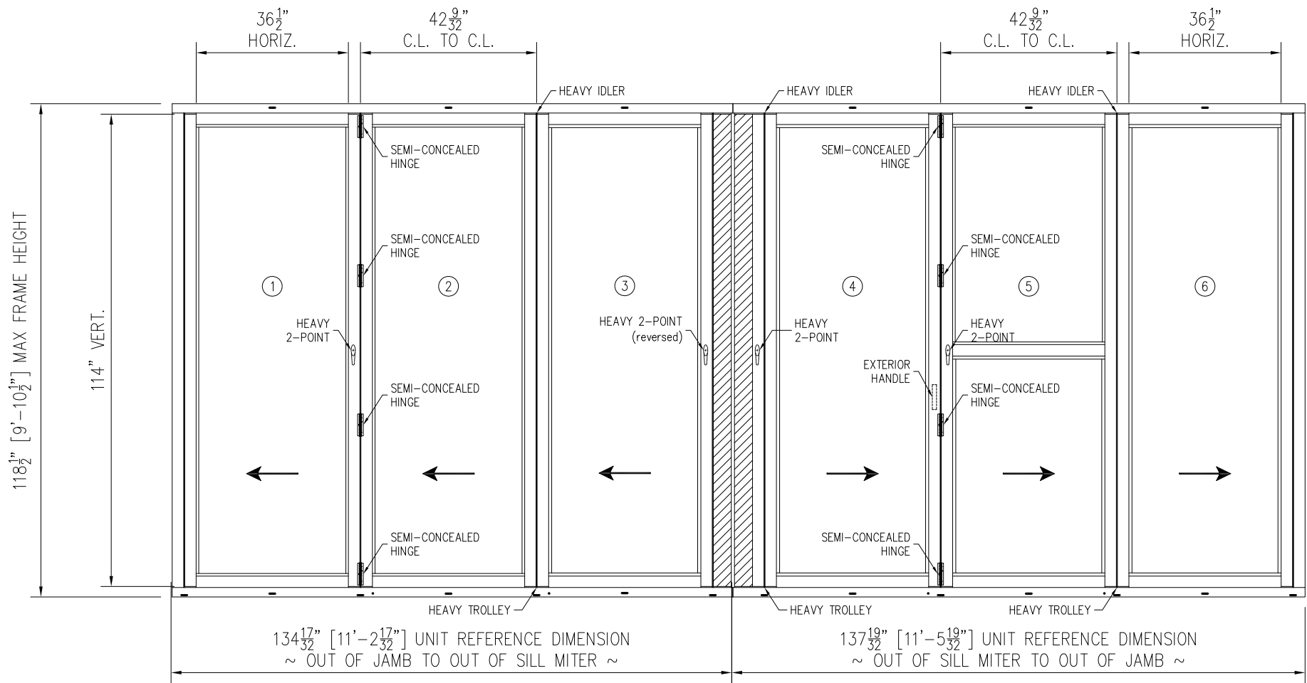
SERIES SI3000 FGW 3.5X9.5 PANEL 90° CORNER NO-POST - STANDARD SILL
