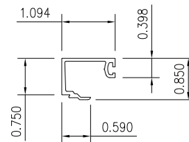
7/16" GLASS STOP
