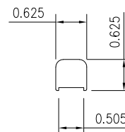
IDLER BODY
