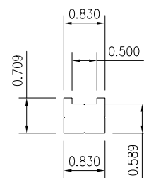
TROLLEY BODY
