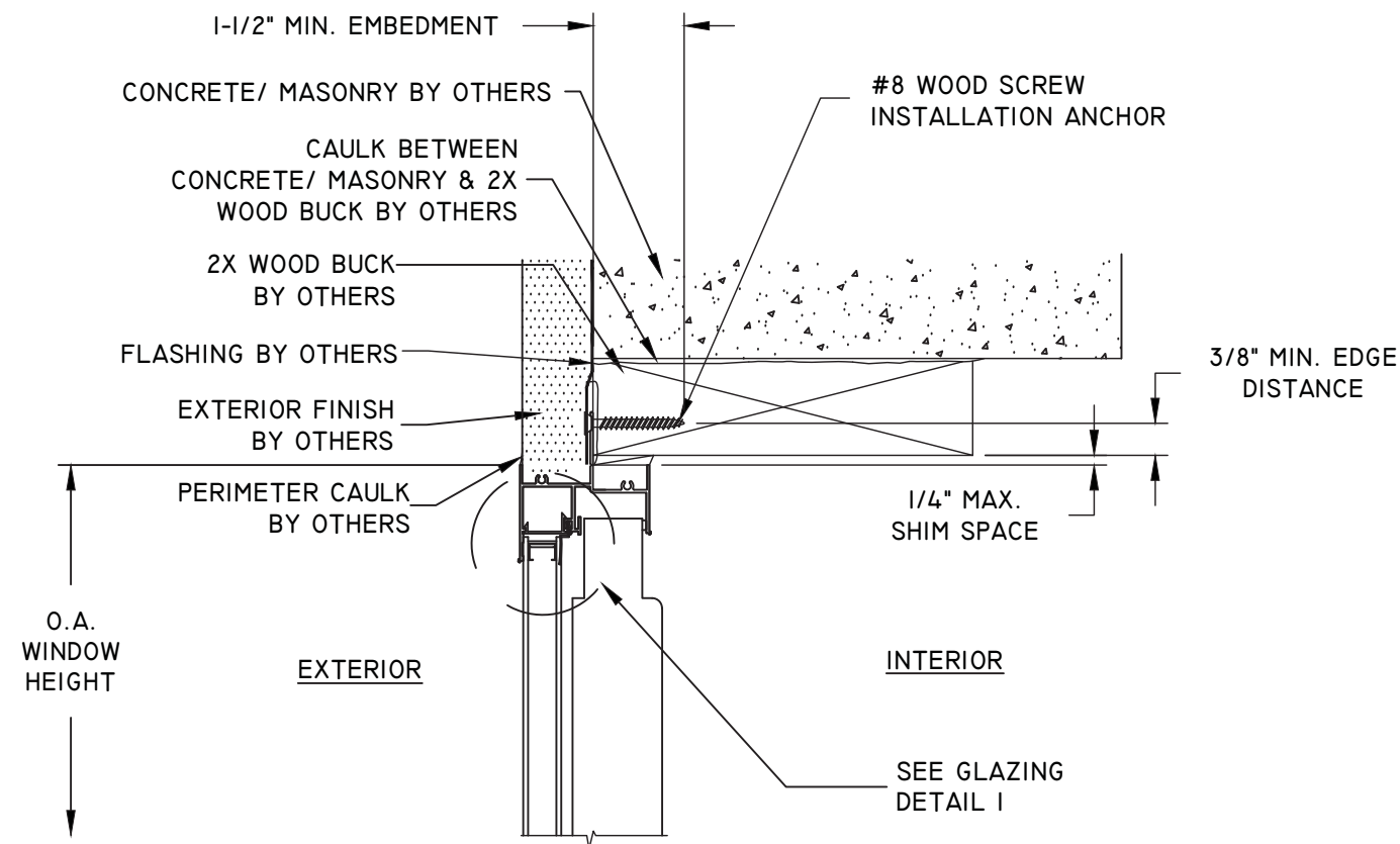
C 3 VERTICAL SECTION HEAD - 2X WOOD BUCK FIN INSTALLATION
