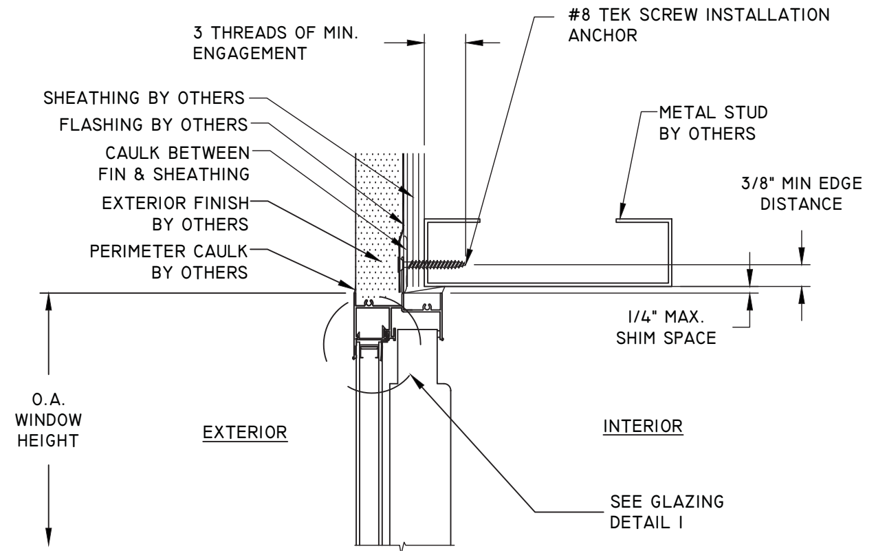
D 3 VERTICAL SECTION HEAD - METAL STUD FIN INSTALLATION
