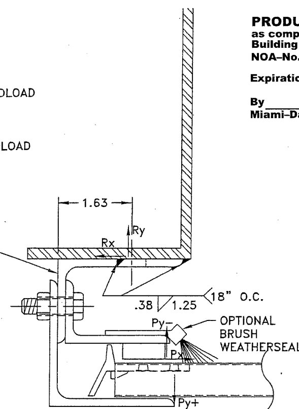
GUIDE MOUNTING DETAIL GUIDES WELDED TO STEEL JAMB AT SLOT AND TOE
