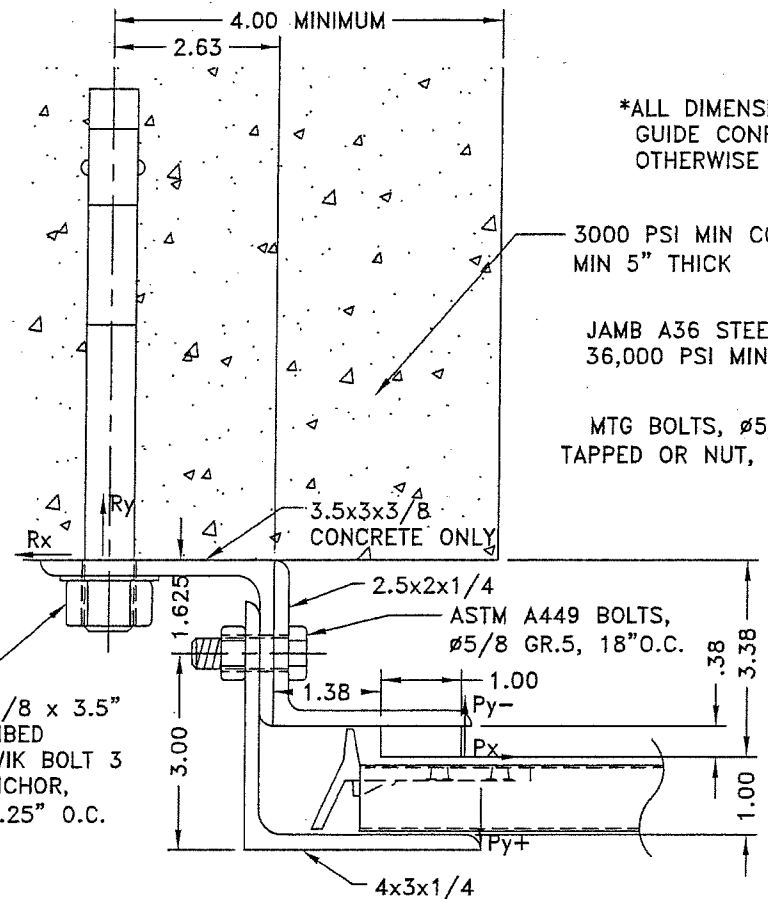
GUIDE MOUNTING DETAIL GUIDES BOLTED TO CONCRETE JAMB
