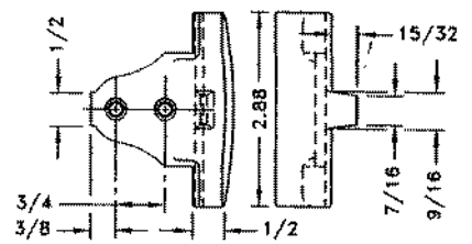
WINDLOCK DETAIL
