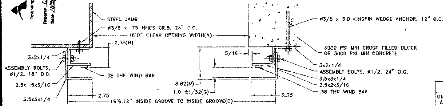
GUIDE DETAIL
