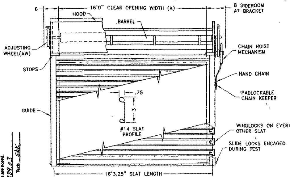
COILSIDE ELEVATION
