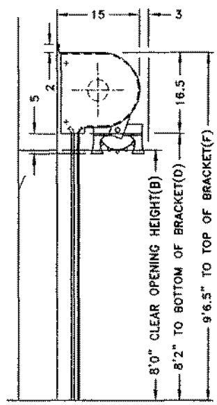
VERTICAL DETAIL
