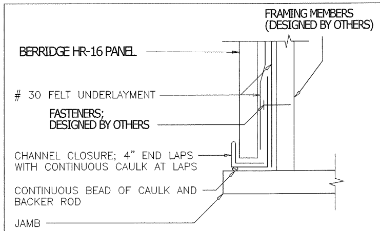
TYPICAL JAMB DETAIL
