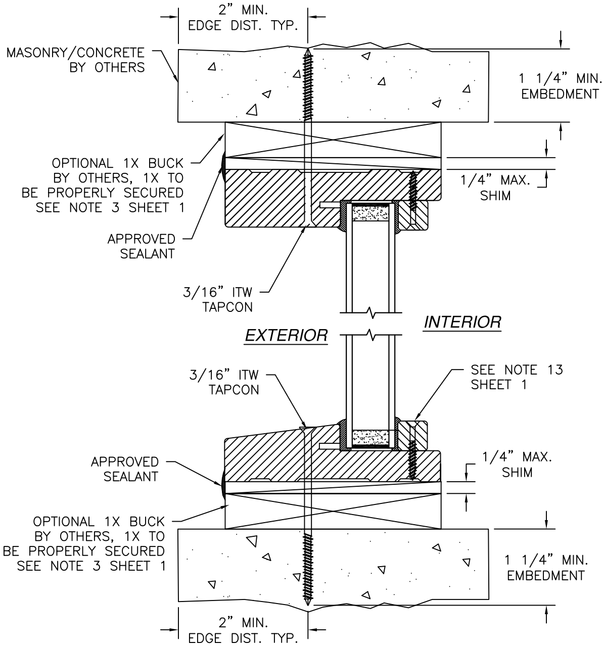
VERTICAL CROSS SECTION MASONRY/CONCRETE INSTALLATION
