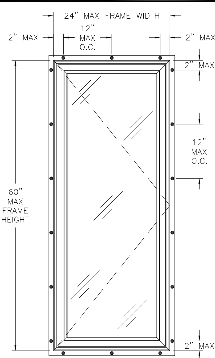
SERIES 1500 OUTSWING CASEMENT EXTERIOR VIEW FIN INSTALLATION
