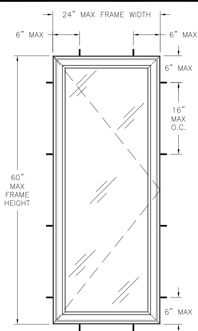
SERIES 1500 OUTSWING CASEMENT EXTERIOR VIEW FRAME INSTALLATION
