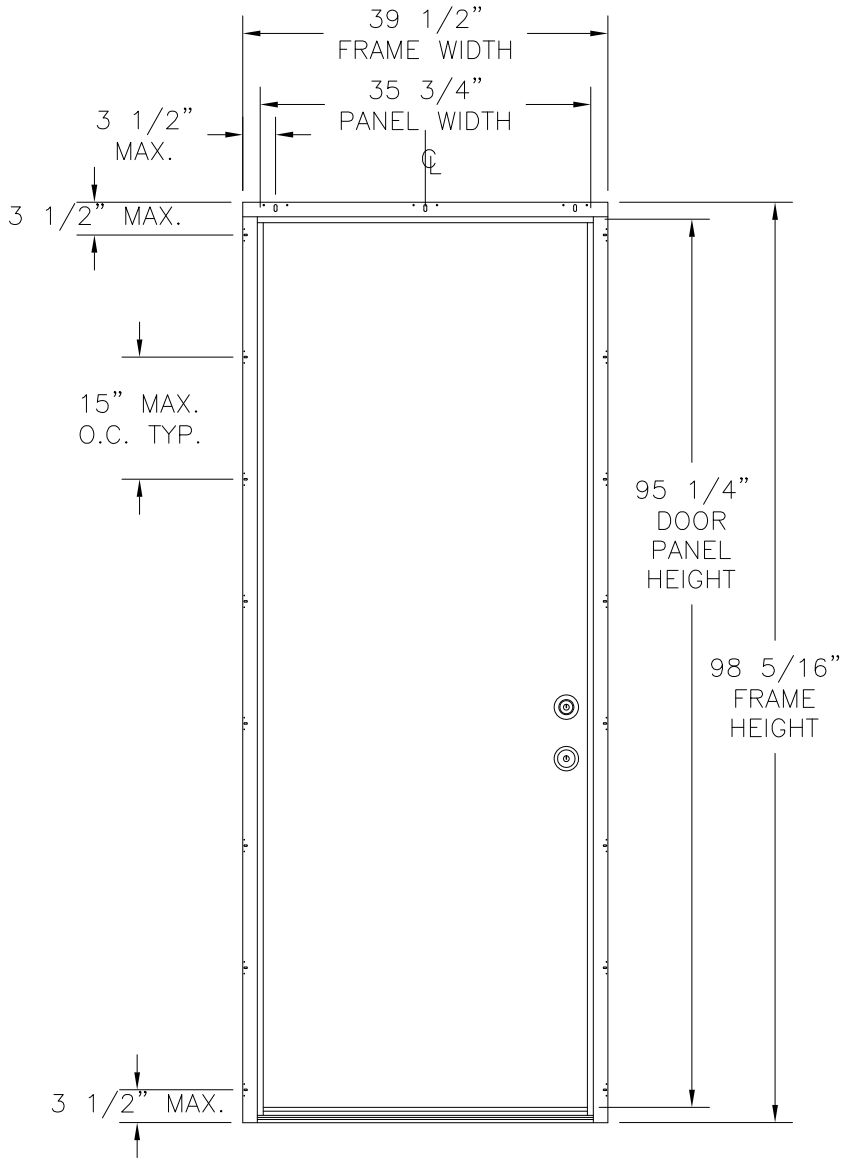
REDIFLEX 18GA. STEEL 2-PIECE FRAME SINGLE DOOR IS/OS EXTERIOR VIEW
