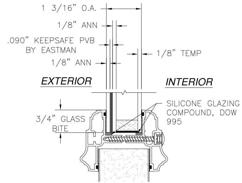
GLAZING DETAIL D
