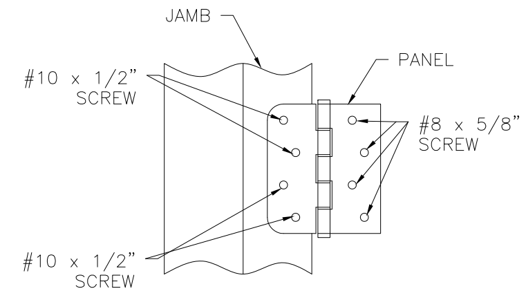
HINGE INSTALLATION DETAIL 2X BUCK/WOOD FRAMING INSTALLATION
