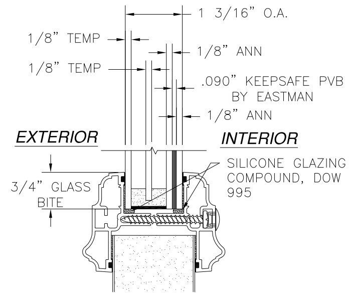
GLAZING DETAIL A
