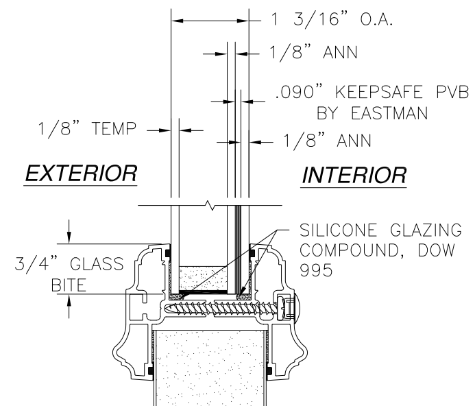
GLAZING DETAIL C
