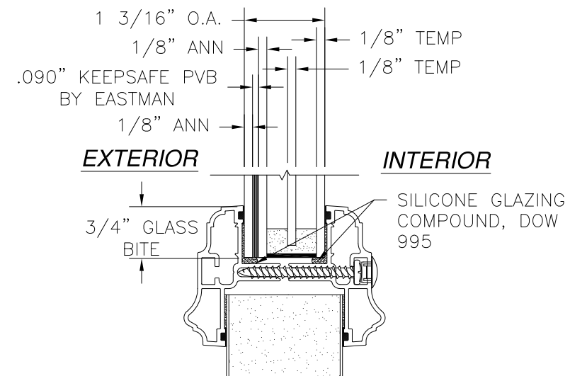
GLAZING DETAIL B
