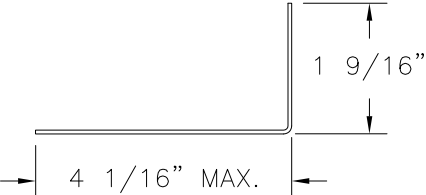
19GA. CLOSER FRAME GALVANIZED SEEL
