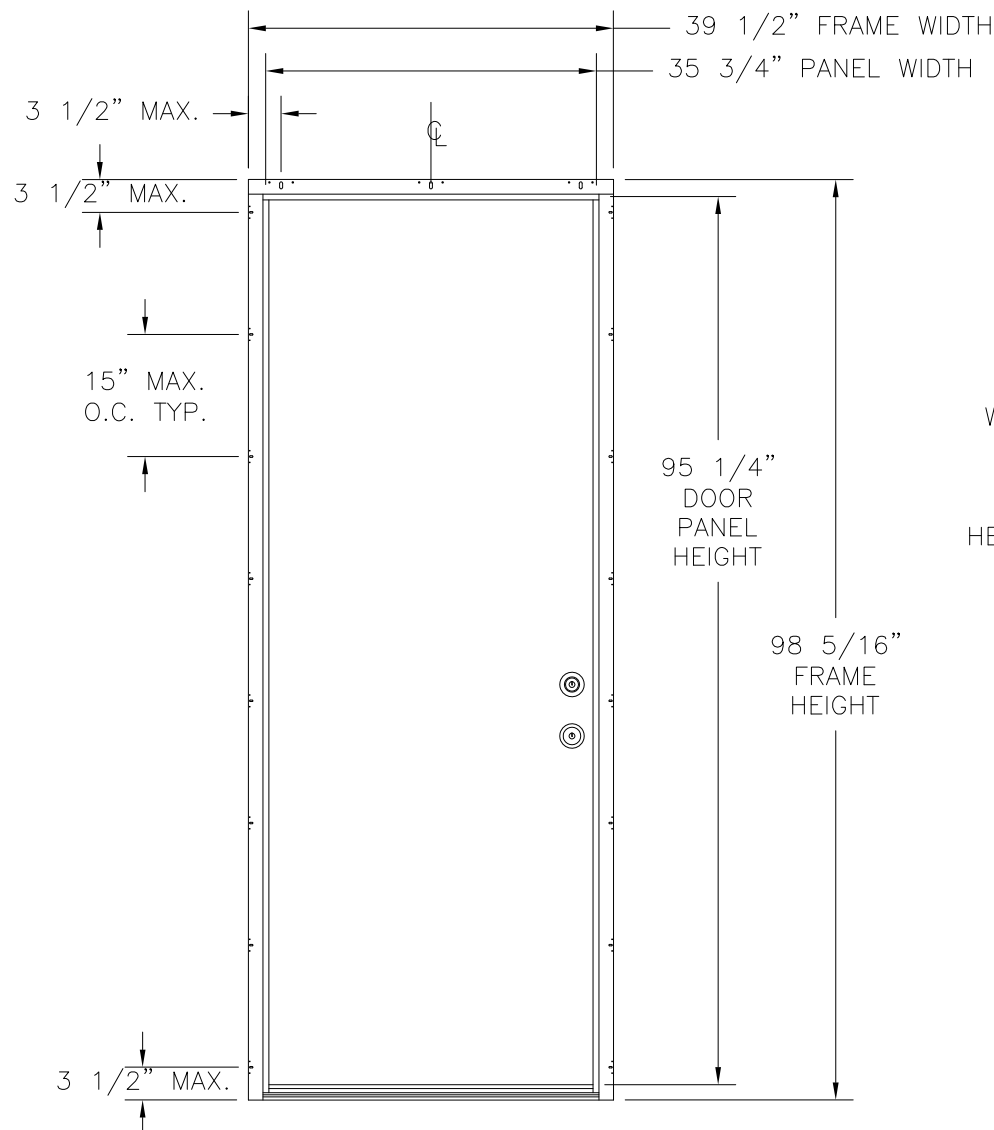
REDIFLEX 18GA. STEEL 2-PIECE FRAME SINGLE DOOR IS/OS EXTERIOR VIEW
