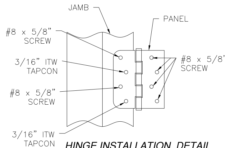
HINGE INSTALLATION DETAIL MASONRY/CONCRETE INSTALLATION
