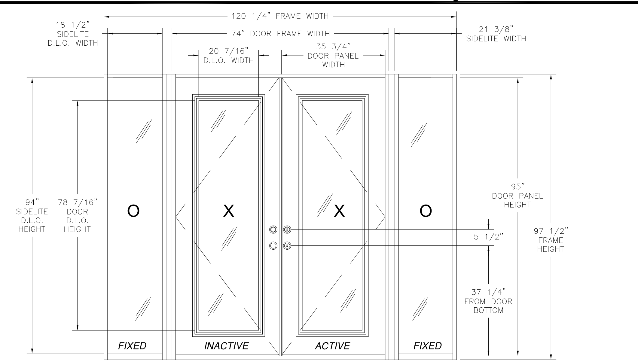
22GA. STEEL DOUBLE DOOR INSWING /OUTSWING W/SIDELITES EXTERIOR VIEW
