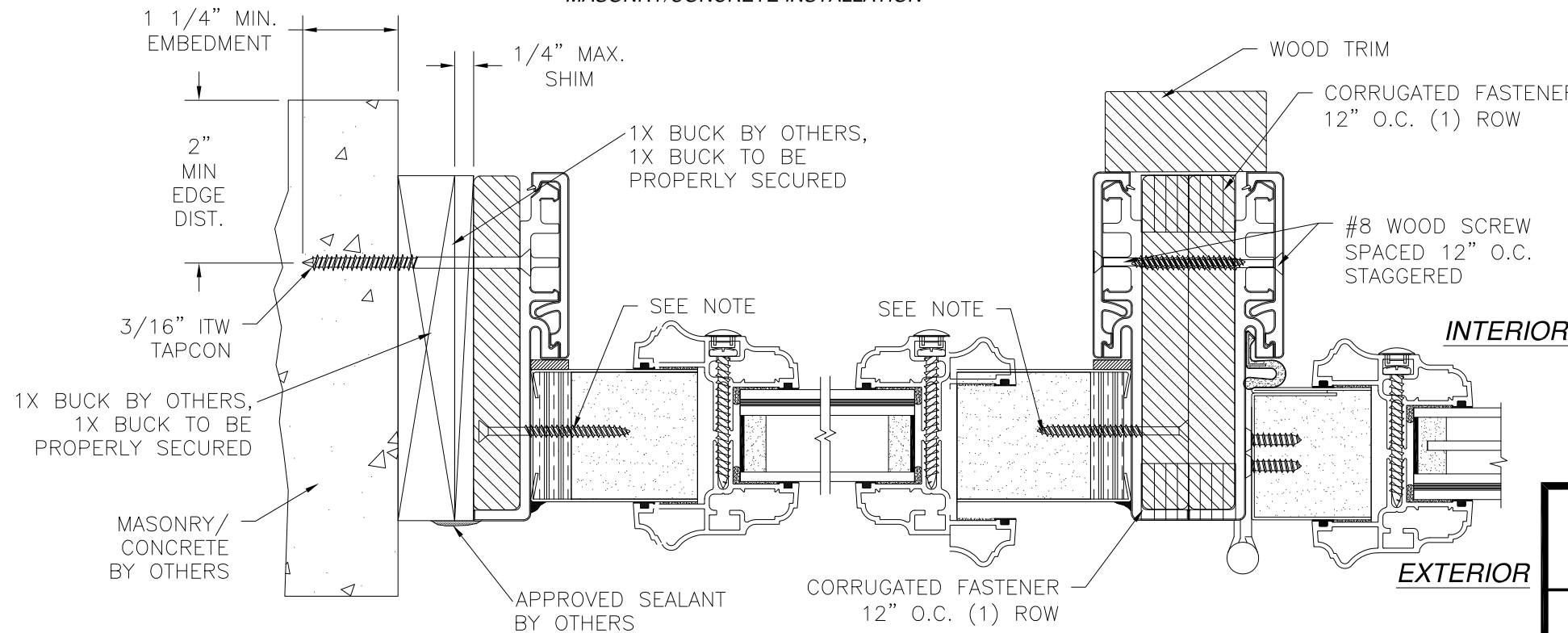
HORIZONTAL CROSS SECTION OUTSWING STANDARD SIDELITE MASONRY/CONCRETE INSTALLATION
