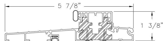
STANDARD OUTSWING SILL
