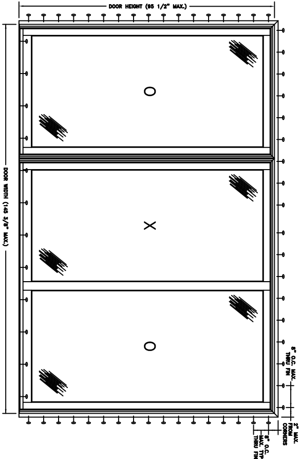
TYPICAL ELEVATION WITH FASTENER SPACING
