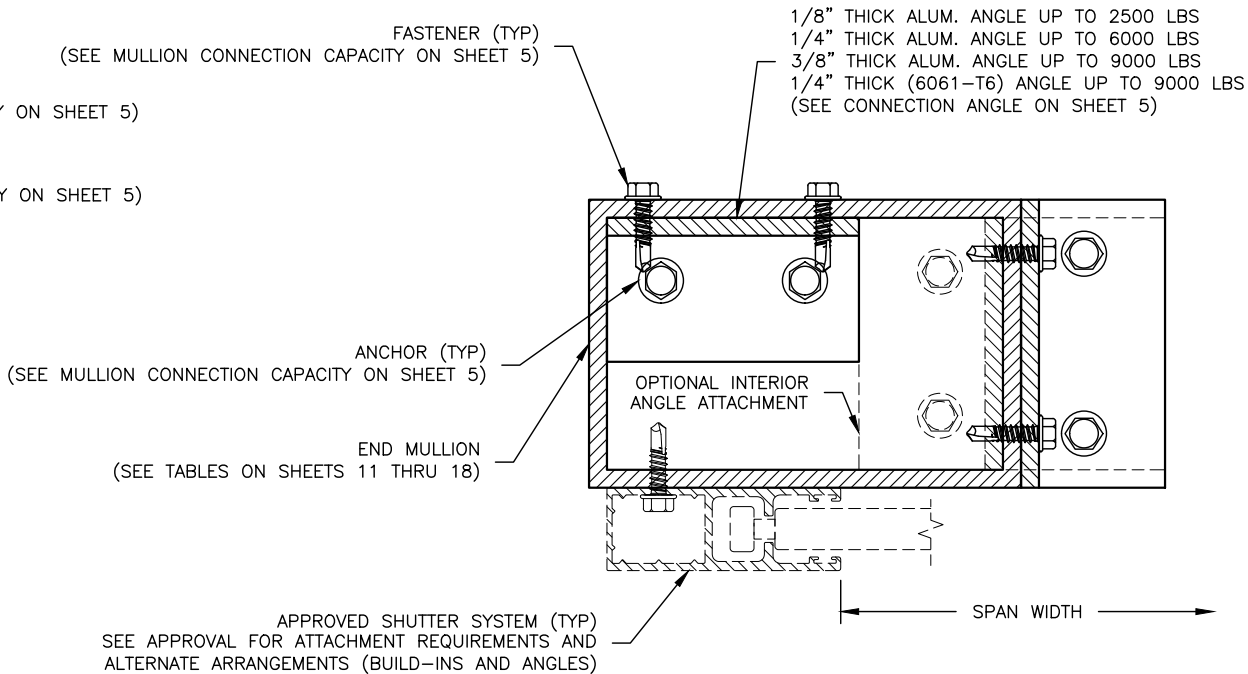
END MULLION CONNECTION INTERIOR ATTACHMENT MULLION INSTALLATION - N.T.S.
