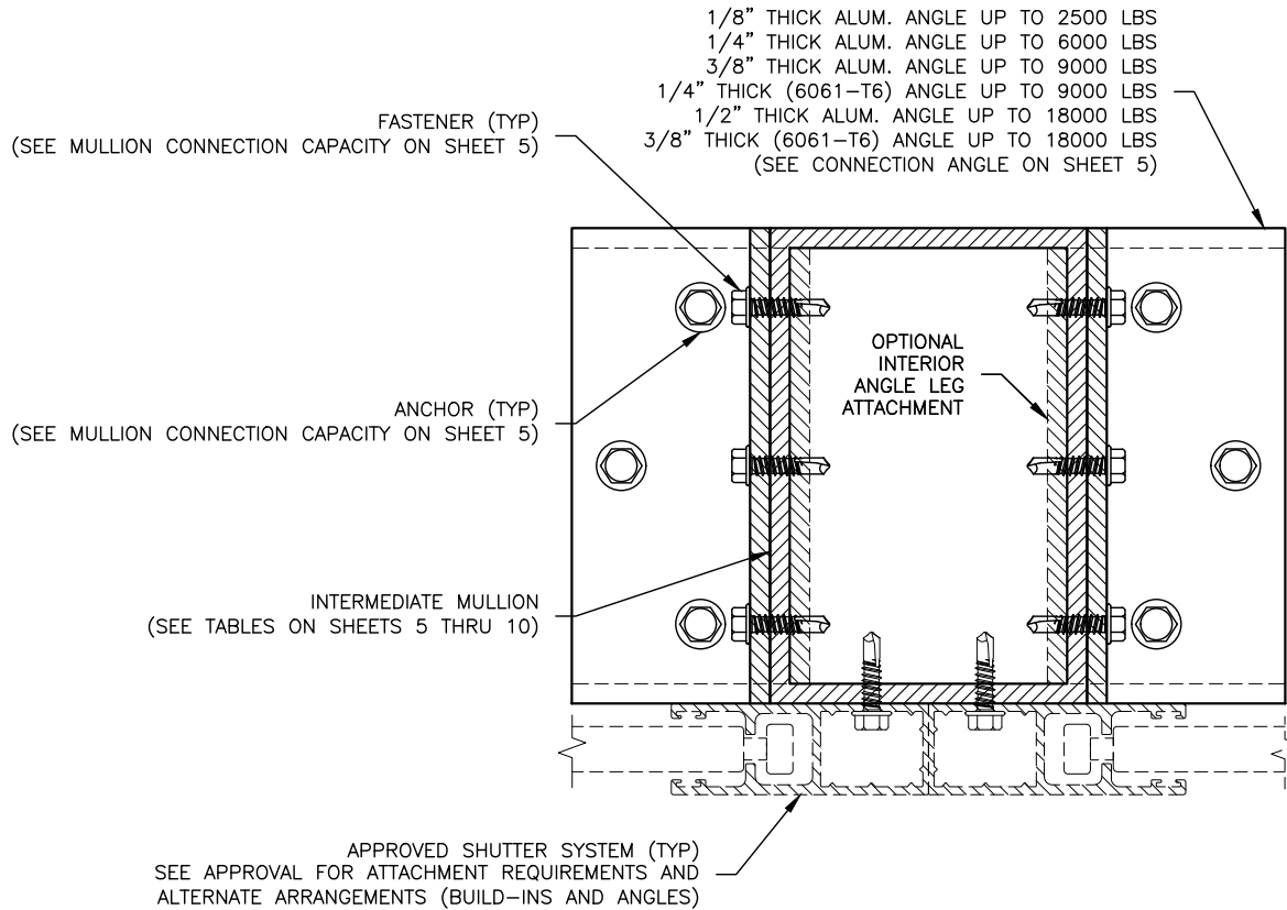
INTERMEDIATE MULLION CONNECTION TYPICAL MULLION INSTALLATION - N.T.S.
