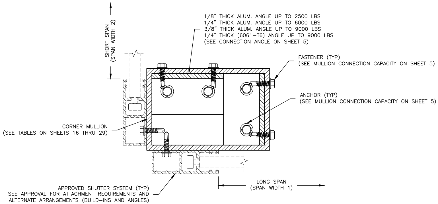
END MULLION CONNECTION INTERIOR ATTACHMENT MULLION INSTALLATION - N.T.S.
