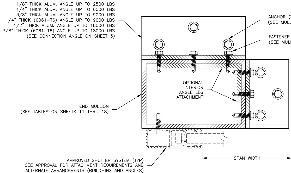
END MULLION CONNECTION TYPICAL MULLION INSTALLATION - N.T.S.
