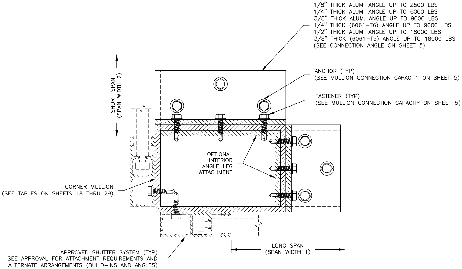
END MULLION CONNECTION TYPICAL MULLION INSTALLATION - N.T.S.
