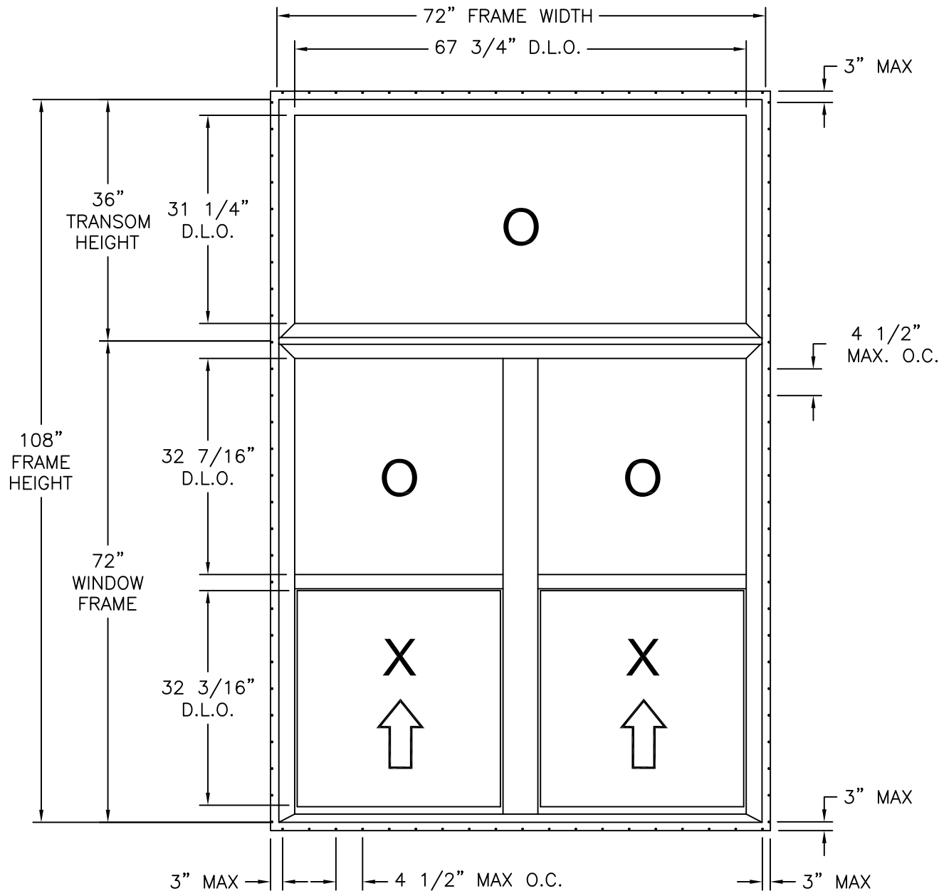
1900 TWIN SINGLE HUNG WITH 1901 TRANSOM EXTERIOR VIEW
