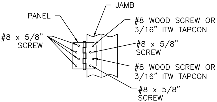
DETAIL A HINGE DETAIL
