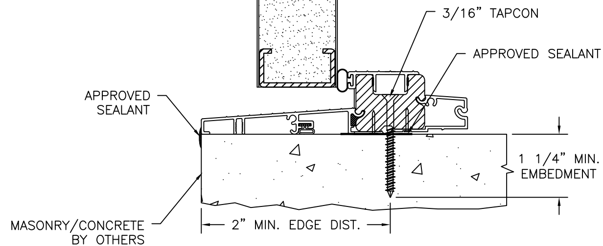
VERTICAL CROSS SECTION OUTSWING STANDARD SILL INSTALLATION MASONRY/CONCRETE INSTALLATION
