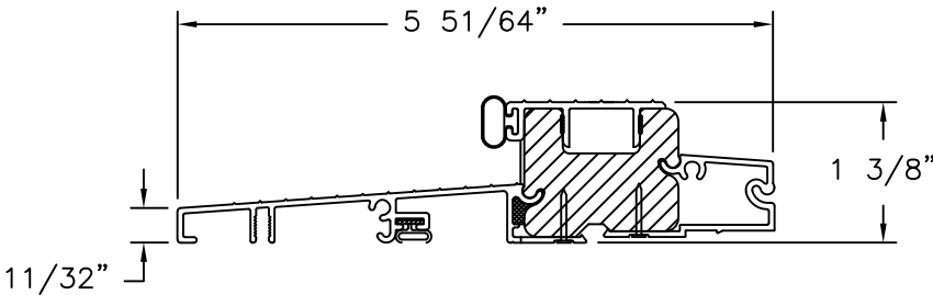
OUTSWING SILL
