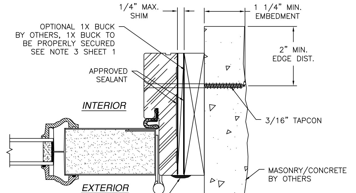
HORIZONTAL CROSS SECTION OUTSWING MASONRY/CONCRETE INSTALLATION HINGE JAMB SHOWN, STRIKE JAMB SIMILAR
