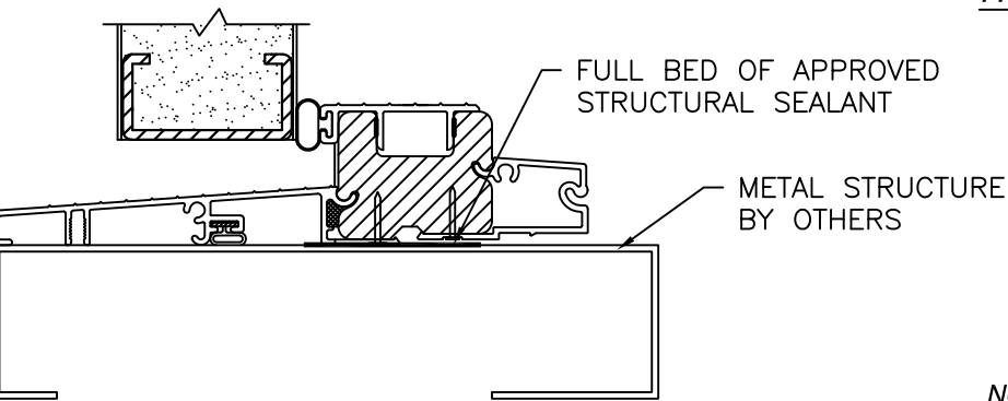
VERTICAL CROSS SECTION OUTSWING
