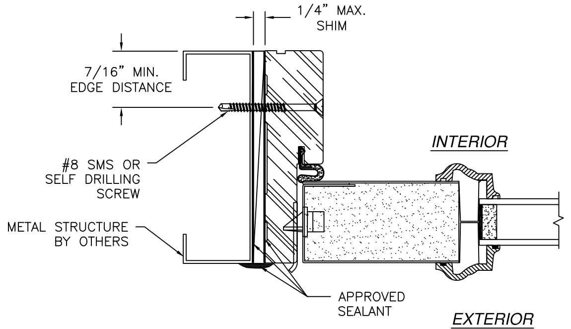
HORIZONTAL CROSS SECTION OUTSWING
