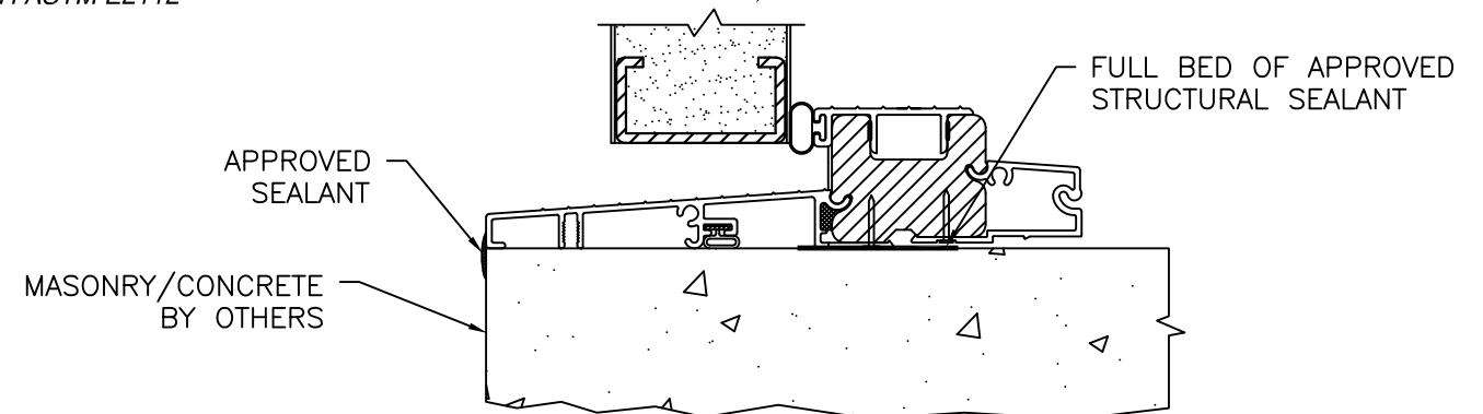
VERTICAL CROSS SECTION OUTSWING OPTIONAL SILL INSTALLATION MASONRY/CONCRETE INSTALLATION
