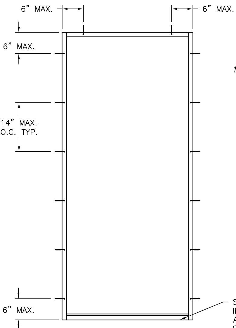
INSWING/OUTSWING ANCHORING LAYOUT OPTIONAL SILL INSTALLATION
