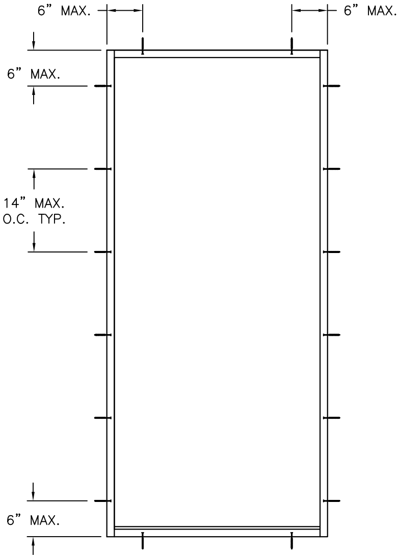
INSWING/OUTSWING ANCHORING LAYOUT STANDARD SILL INSTALLATION
