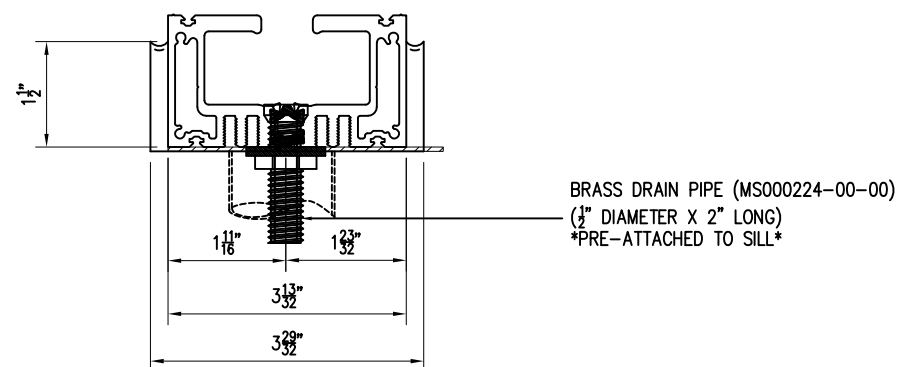
DRAIN PIPE DETAIL WITH FLUSH SILL
