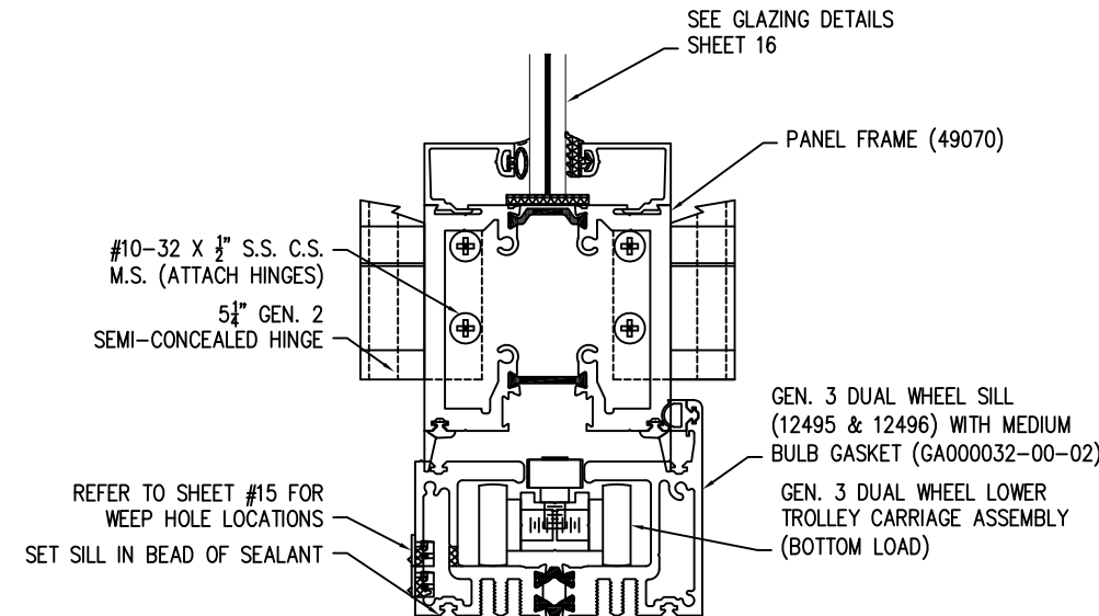
VERTICAL CROSS SECTION BOTTOM LOAD SILL WITH STANDARD SILL
