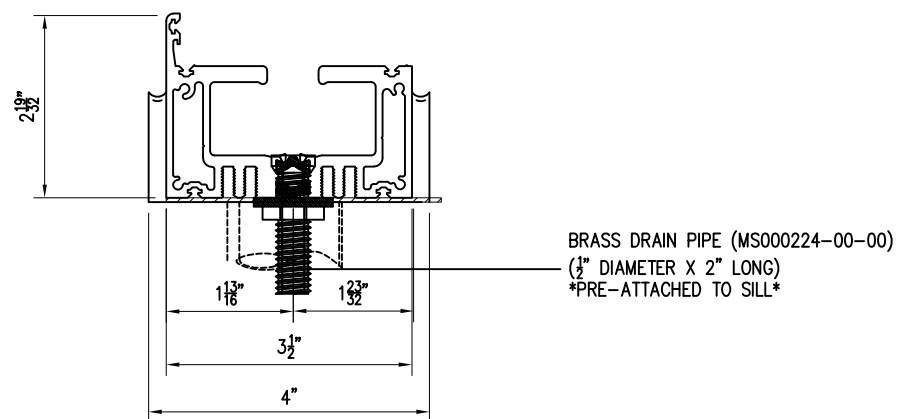
DRAIN PIPE DETAIL WITH STANDARD SILL
