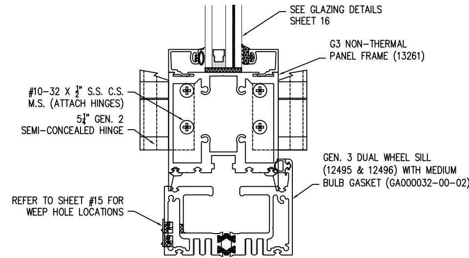
VERTICAL CROSS SECTION NON-THERMAL PANEL WITH STANDARD SILL
