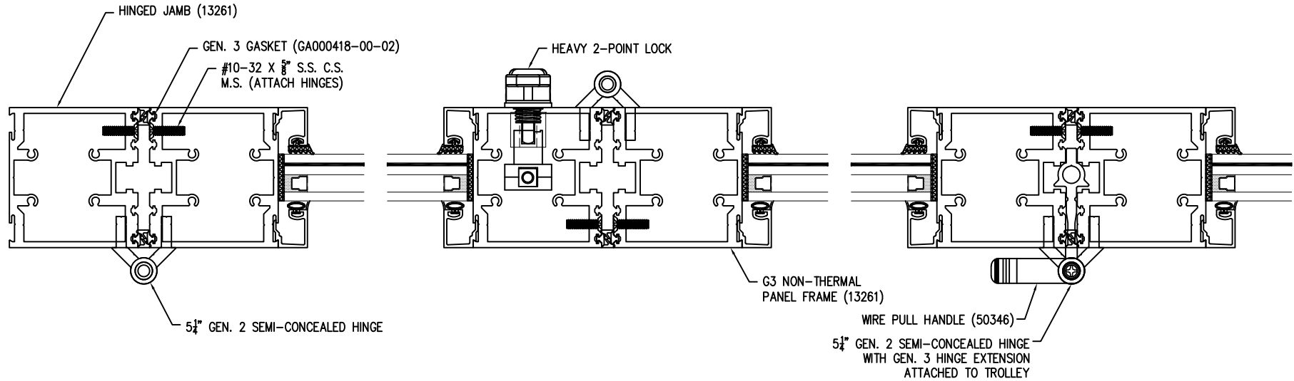
HORIZONTAL CROSS SECTION WITH NON-THERMAL FRAME
