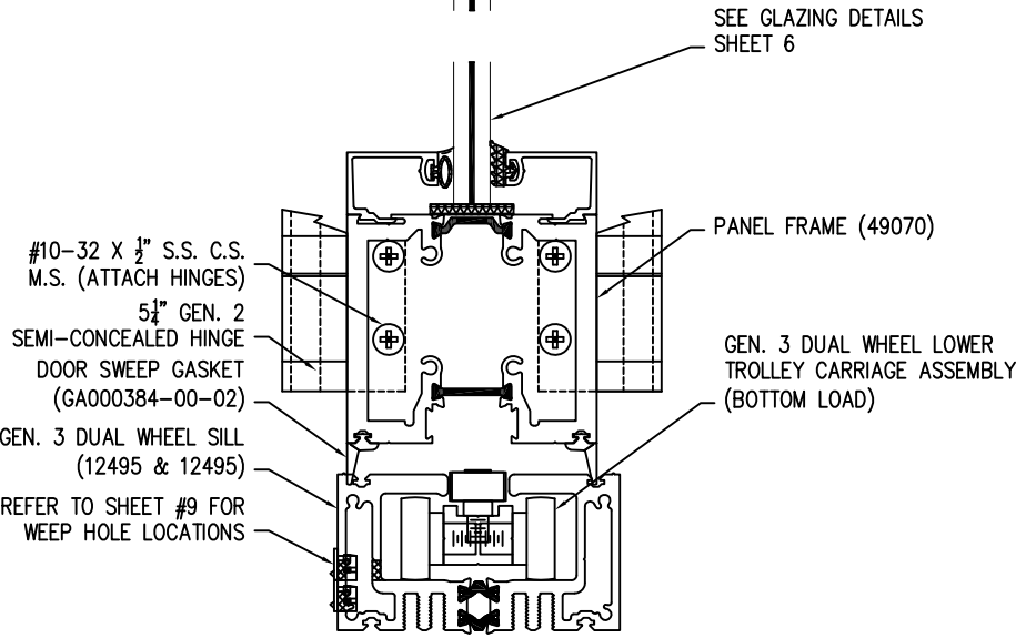
VERTICAL CROSS SECTION BOTTOM LOAD SILL
