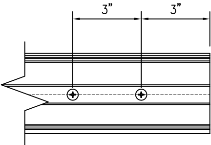
SILL AND HEAD END DETAIL
