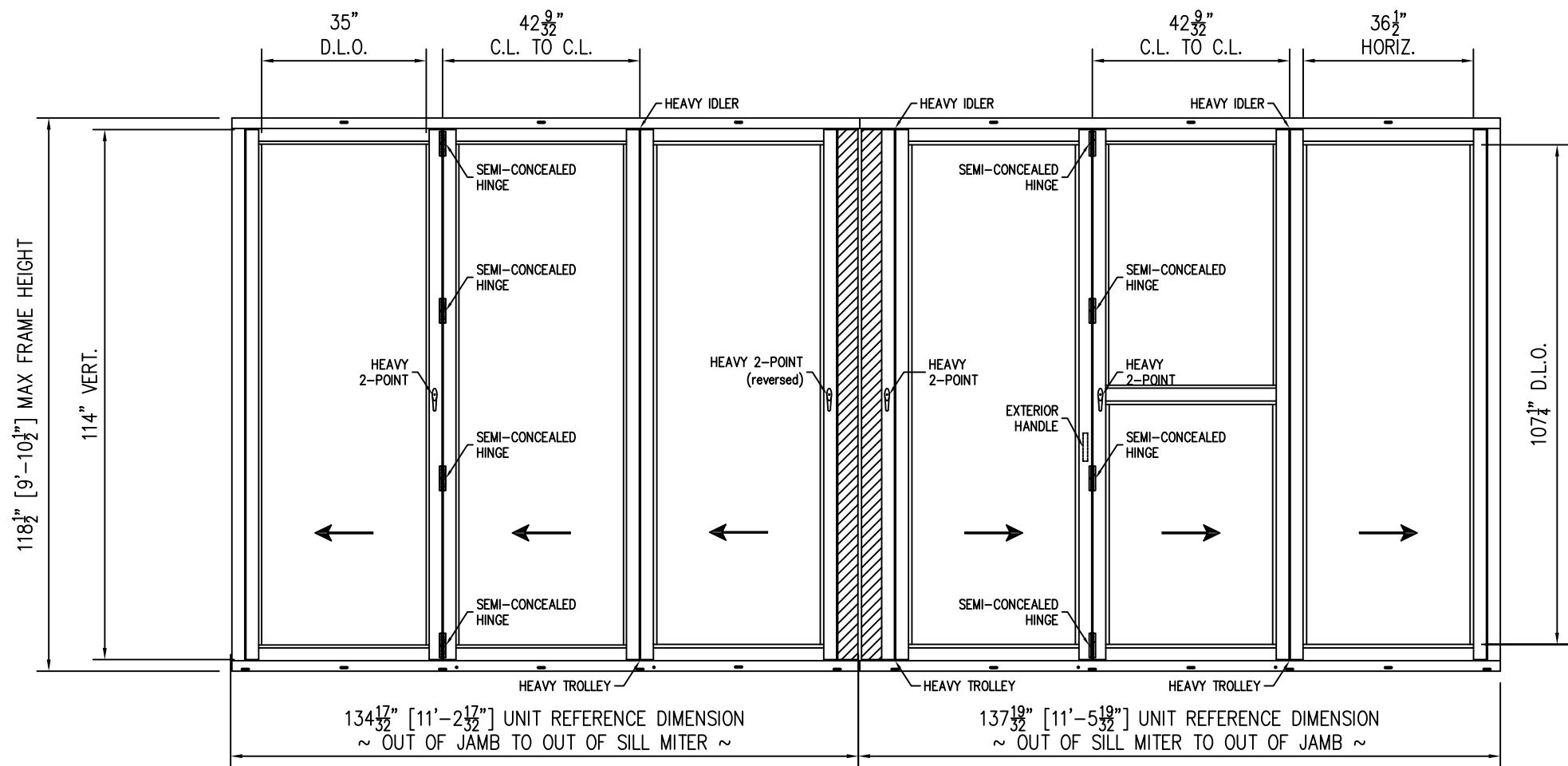
SERIES SI3000 G3 IMPACT FGW 3.5X9.5 PANEL 90° CORNER NO-POST - FLUSH SILL
