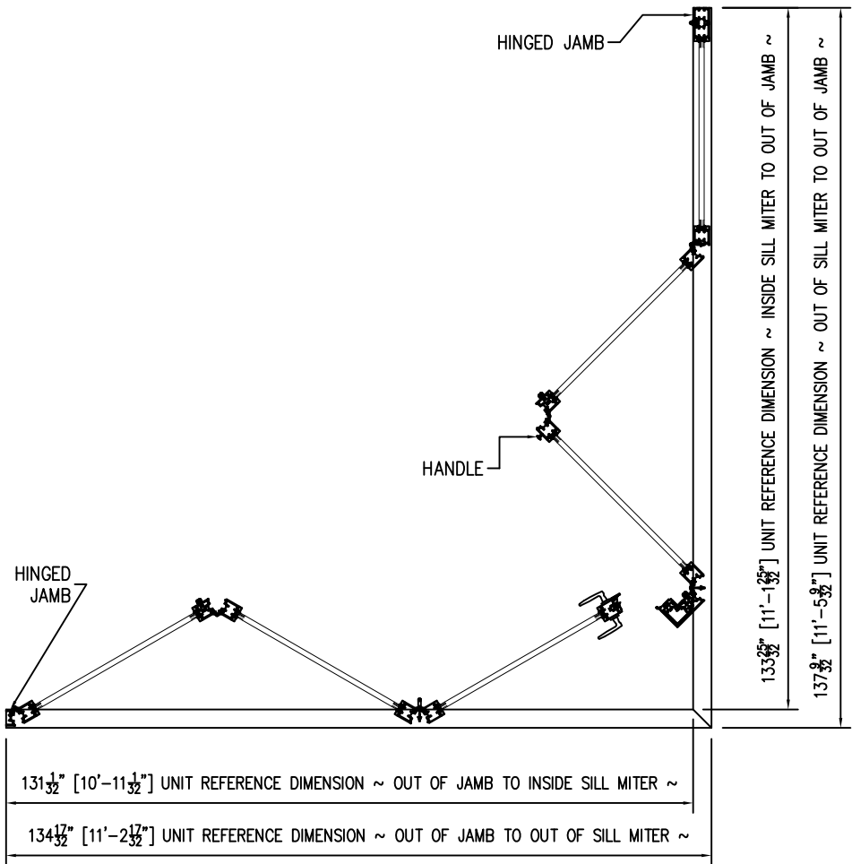
SI 33350 G3 IMPACT FGW 3.5X9.5 PANEL 90° CORNER NO-POST - FLUSH SILL
