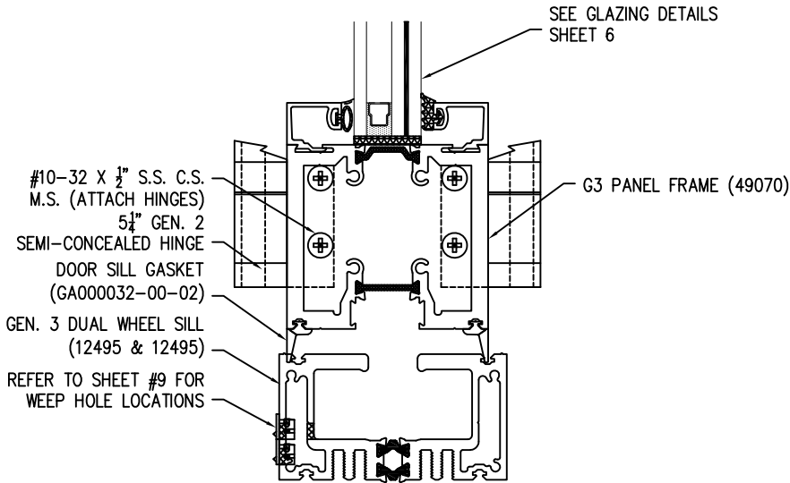
VERTICAL CROSS SECTION STANDARD
