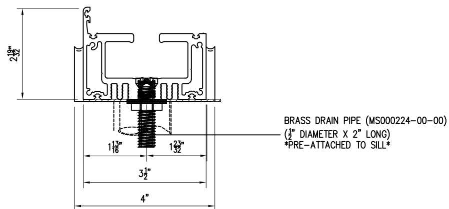
DRAIN PIPE DETAIL
