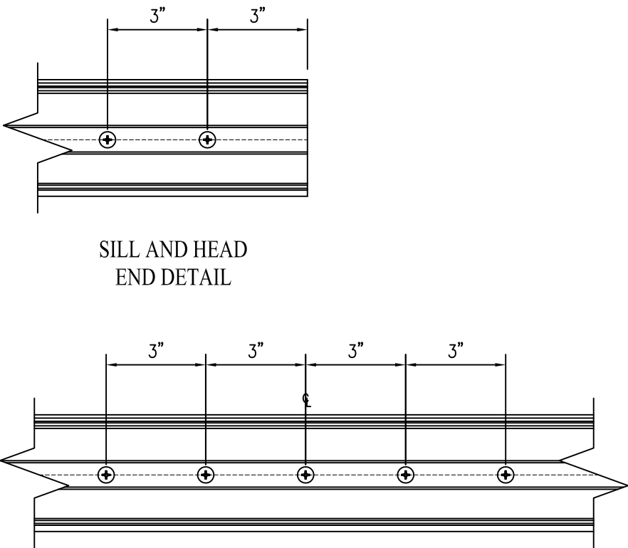
SILL AND HEAD CLUSTER DETAIL
