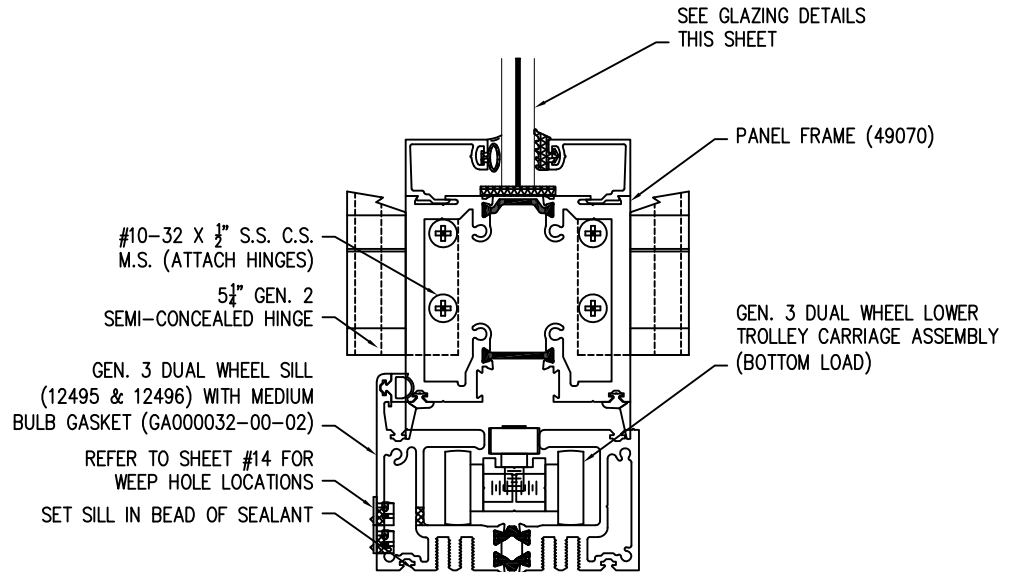
VERTICAL CROSS SECTION BOTTOM LOAD SILL
