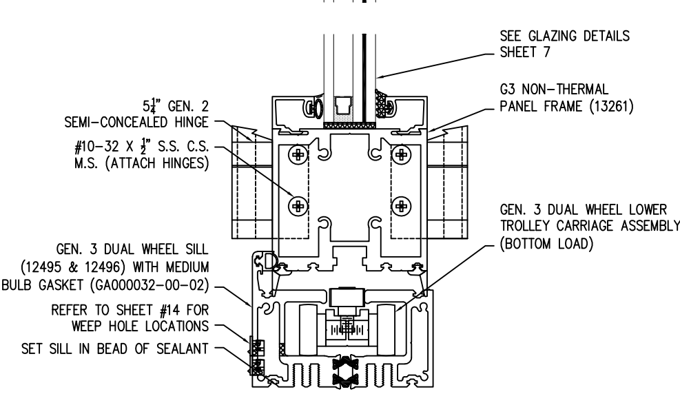
VERTICAL CROSS SECTION NON-THERMAL PANEL
