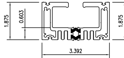
FLUSH SILL
