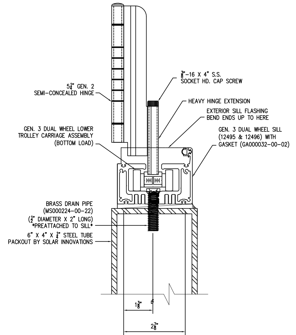
DRAIN PIPE AND HINGE EXTENSION DETAILS
