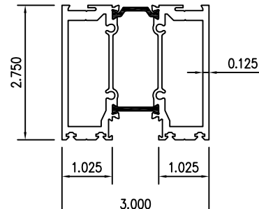
LIGHT THERMAL FRAME
