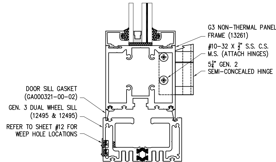
VERTICAL CROSS SECTION NON-THERMAL PANELS WITH FLUSH SILL
