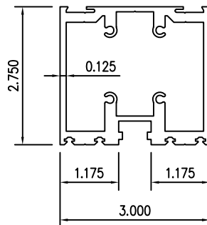
NON-THERMAL FRAME
