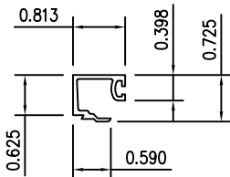
1/4" GLASS STOP
