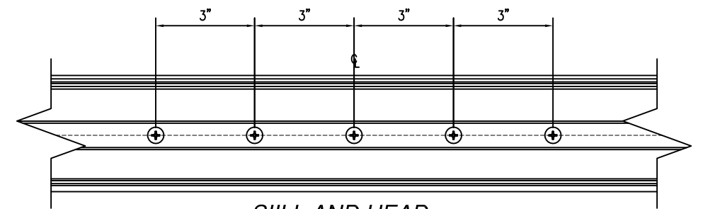
SILL AND HEAD CLUSTER DETAILS
