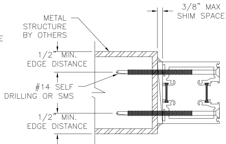
JAMB INSTALLATION DETAIL METAL STRUCTURE
