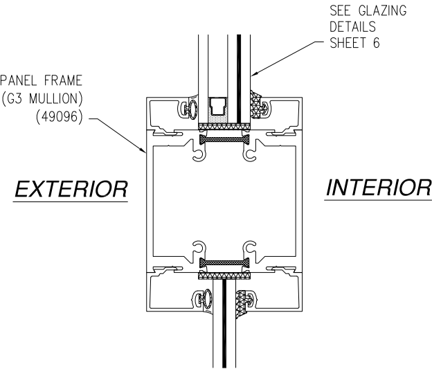
VERTICAL CROSS SECTION HORIZONTAL RAIL OPTIONAL
