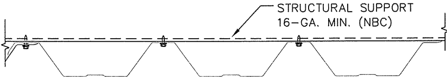
MR3-36 (3 FASTENER PER PANEL WIDTH)
