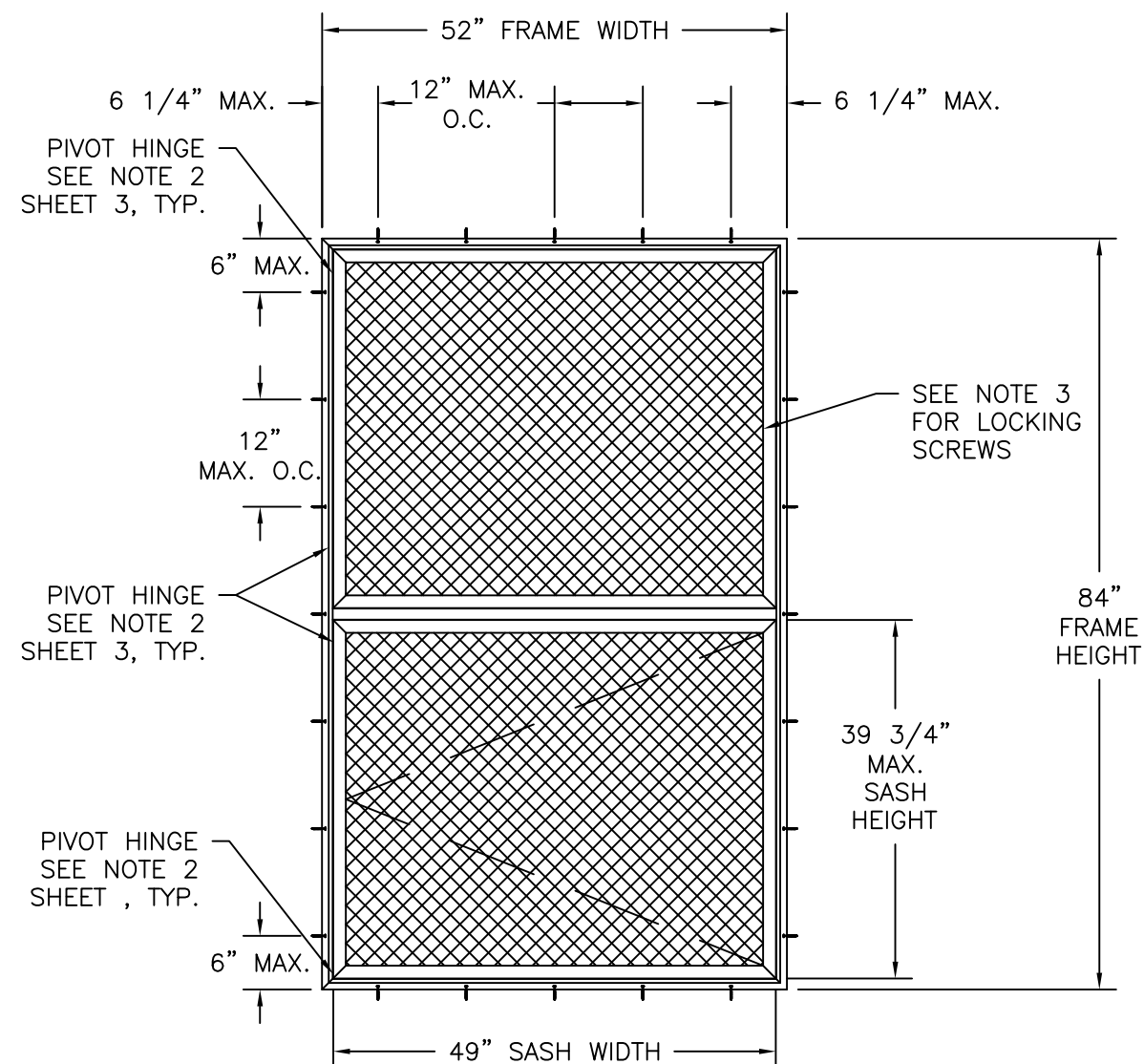
200-13 SIDE PIVOT MULLED ALUMINUM SCREEN EXTERIOR VIEW
