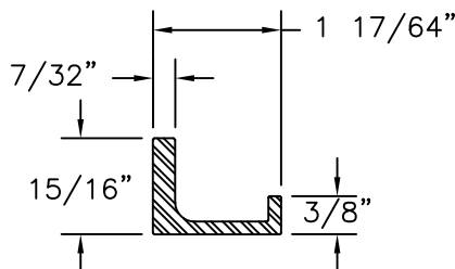
HS FILLER ALUMINUM 6005-T6 .125" THICK
