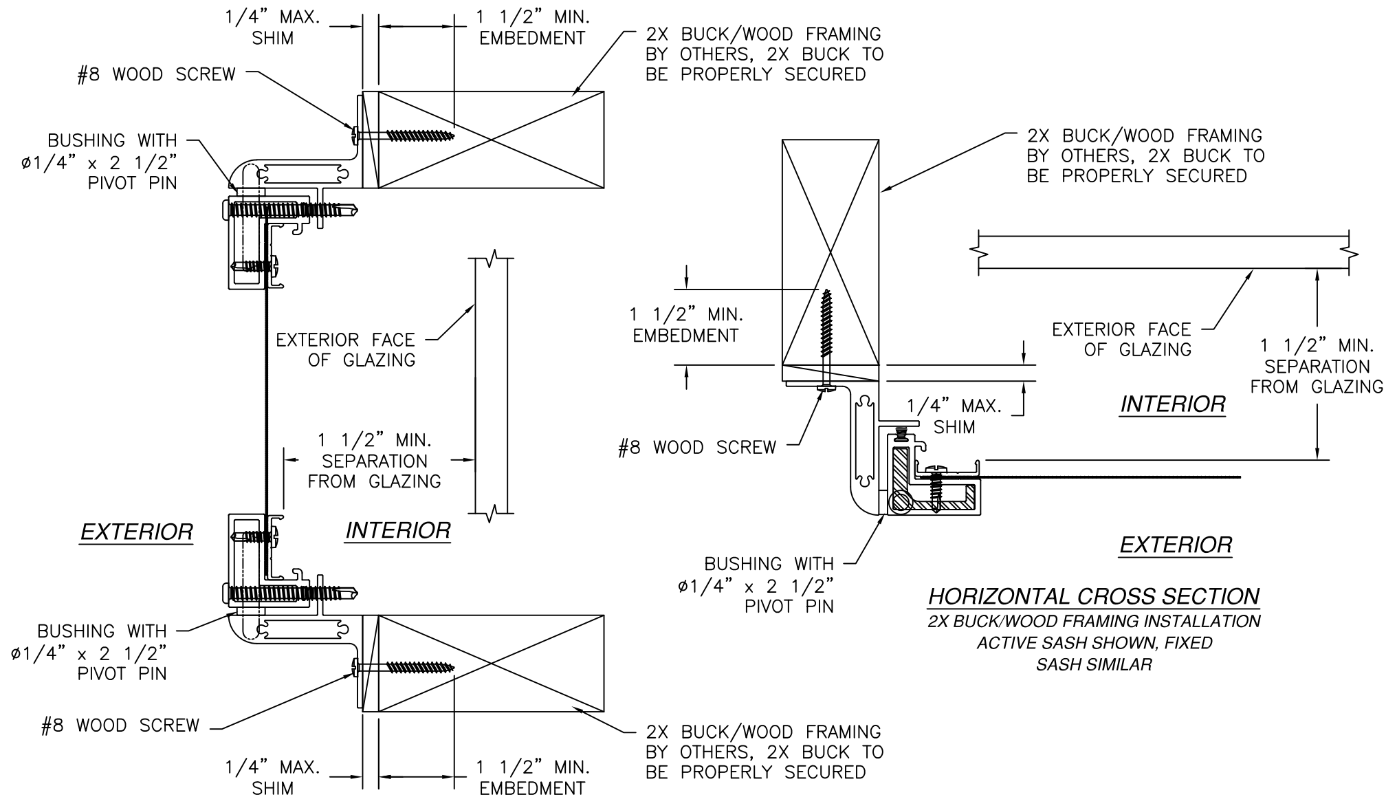
VERTICAL CROSS SECTION 2X BUCK/WOOD FRAMING INSTALLATION SINGLE SCREEN SHOWN, MULLER SCREEN SIMILAR
