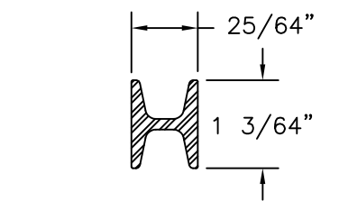
SUPPORT I-BEAM ALUMINUM 6005-T6 .125" THICK
