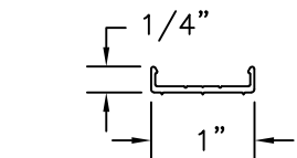
FLAT BAR U-CHANNEL ALUMINUM 6063-T5 .060" THICK
