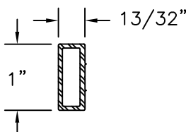
MULLION ALUMINUM 6063-T5 .075" THICK
