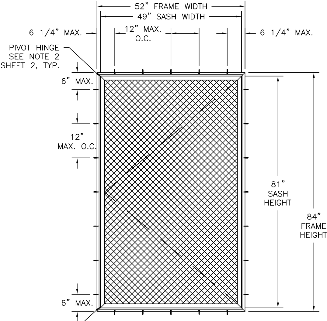
200-12 SIDE PIVOT ALUMINUM SCREEN EXTERIOR VIEW
