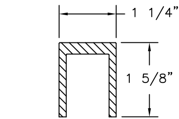
U-CHANNEL ALUMINUM 6005-T6 .156" THICK
