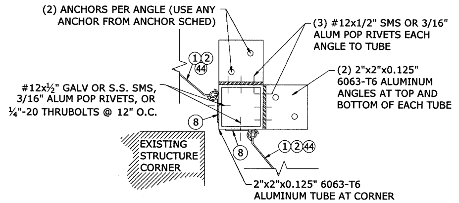
5 6 STANDARD CORNER CLOSURE N.T.S. HORIZ SECTION
