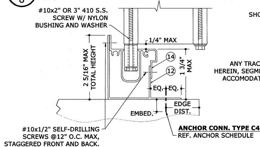
4 ALT. ADJUSTABLE SILL TRACK 8 THRU-FLANGE INSTALLATION N.T.S. VERT SECTION
