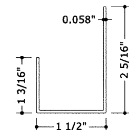
11 ADJUSTABLE SILL TRACK BOTTOM N.T.S. 6063-T6
