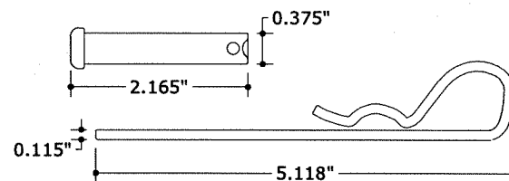
28 CLEVIS AND PIN N.T.S. CADMIUM PLATED STEEL
