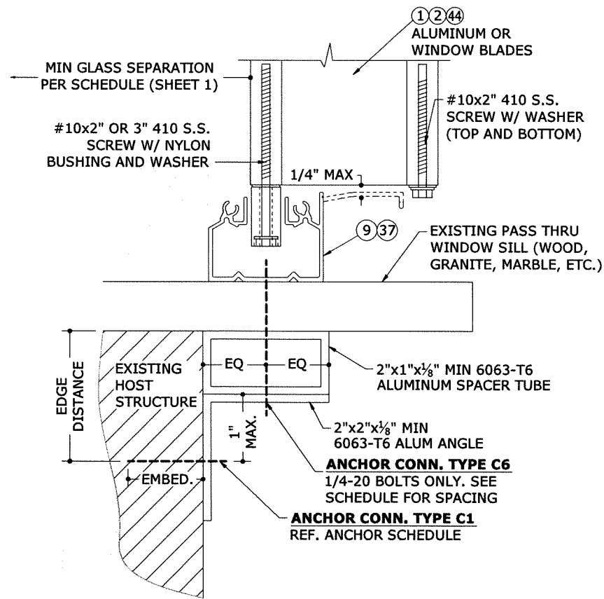
4 6 PASS THRU WINDOW DETAIL N.T.S. VERT SECTION
