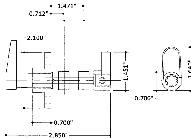
23 LOCK ASSEMBLY N.T.S. ZINC ALLOY/STAINLESS STEEL
