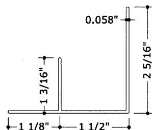
12 ALT. ADJUSTABLE SILL TRACK BOTTOM N.T.S. 6063-T6
