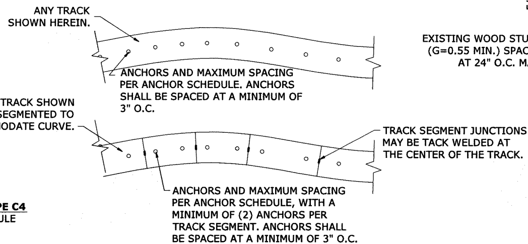
5 OPTIONAL CURVED TRACK 8 W/ & W/O SEGMENTED SECTIONS N.T.S. PLAN VIEW
