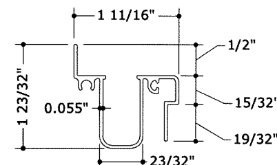
14 ADJUSTABLE SILL TRACK TOP N.T.S. 6063-T6
