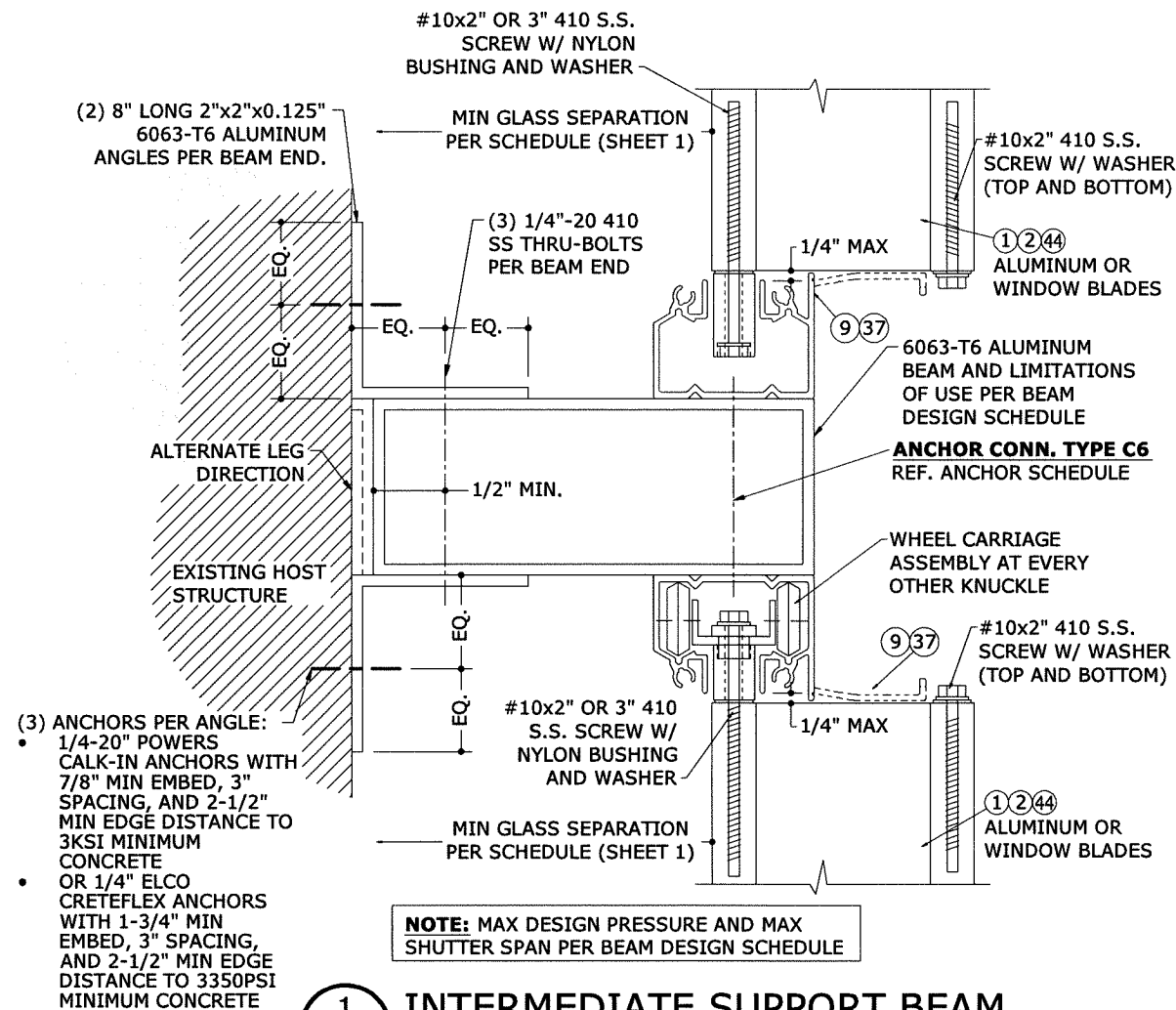
1 10 N.T.S. INTERMEDIATE SUPPORT BEAM VERT SECTION
