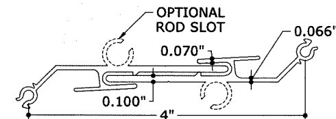
40 ALT. HERMAPHRODITIC CENTERMATE N.T.S. 6063-T6
