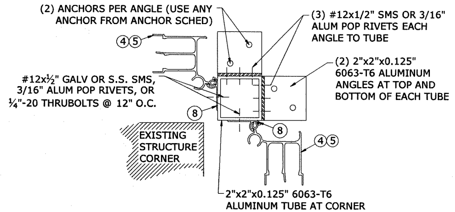
6 6 ALTERNATE CORNER CLOSURE N.T.S. HORIZ SECTION
