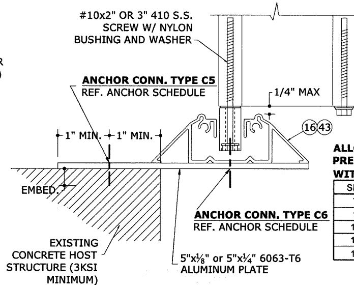
2 10 N.T.S. 5"x1/4" OR 5"x1/8" PLATE TO EXISTING HOST STRUCTURE VERT SECTION
