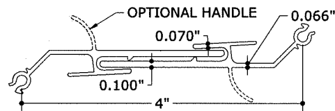
3 HERMAPHRODITIC CENTERMATE N.T.S. 6063-T6
