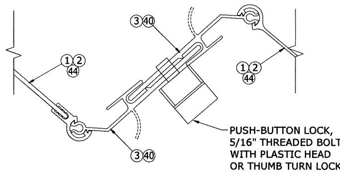
2 6 ALT. HERMAPHRODITIC CENTERMATE N.T.S. HORIZ SECTION
