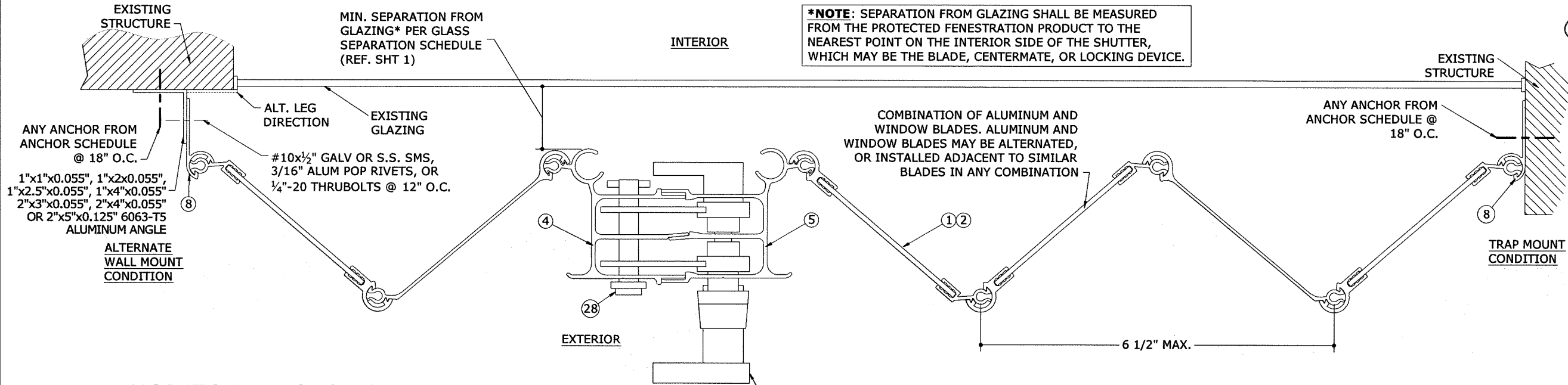
1 6 HORIZONTAL SECTION W/ COMBINATION BLADES N.T.S. HORIZ SECTION
