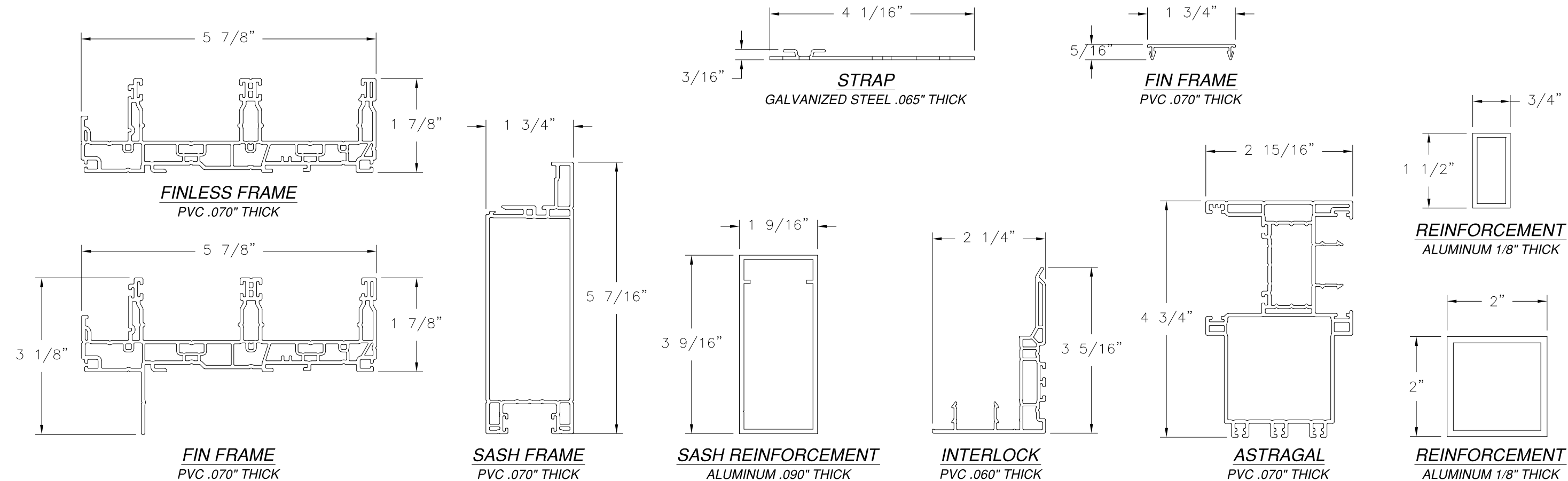
HORIZONTAL CROSS SECTION FOR REFERENCE ONLY, SEE SHEETS 4-11 FOR INSTALLATION DETAILS
