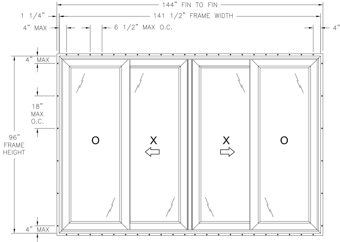
SERIES 9700 VINYL SGD OXXO EXTERIOR VIEW FIN INSTALLATION FOR RATINGS AND NOTES SEE SHEET 2
