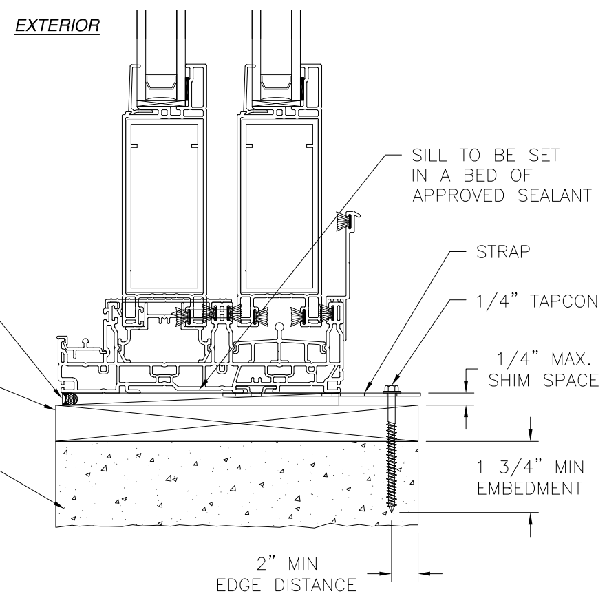
VERTICAL CROSS SECTION CONCRETE/MASONRY INSTALLATION
