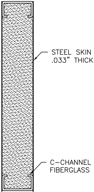
20GA STEEL
