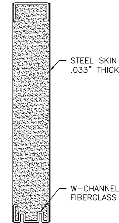
20GA STEEL
