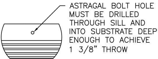
ASTRAGAL SILL DETAIL
