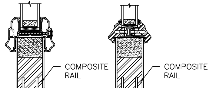
OPTION 29 STANDARD TRIM
