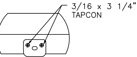
ASTRAGAL HEAD STRIKE DETAIL MASONRY/CONCRETE
