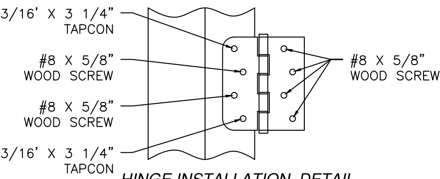
HINGE INSTALLATION DETAIL MASONRY/CONCRETE
