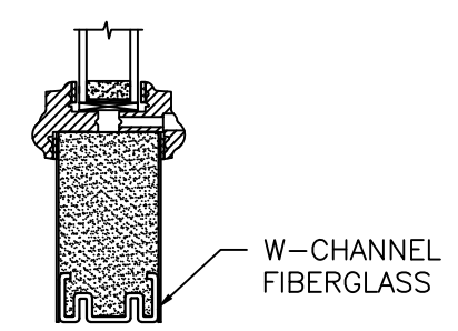
OPTION 14 XLE TRIM
