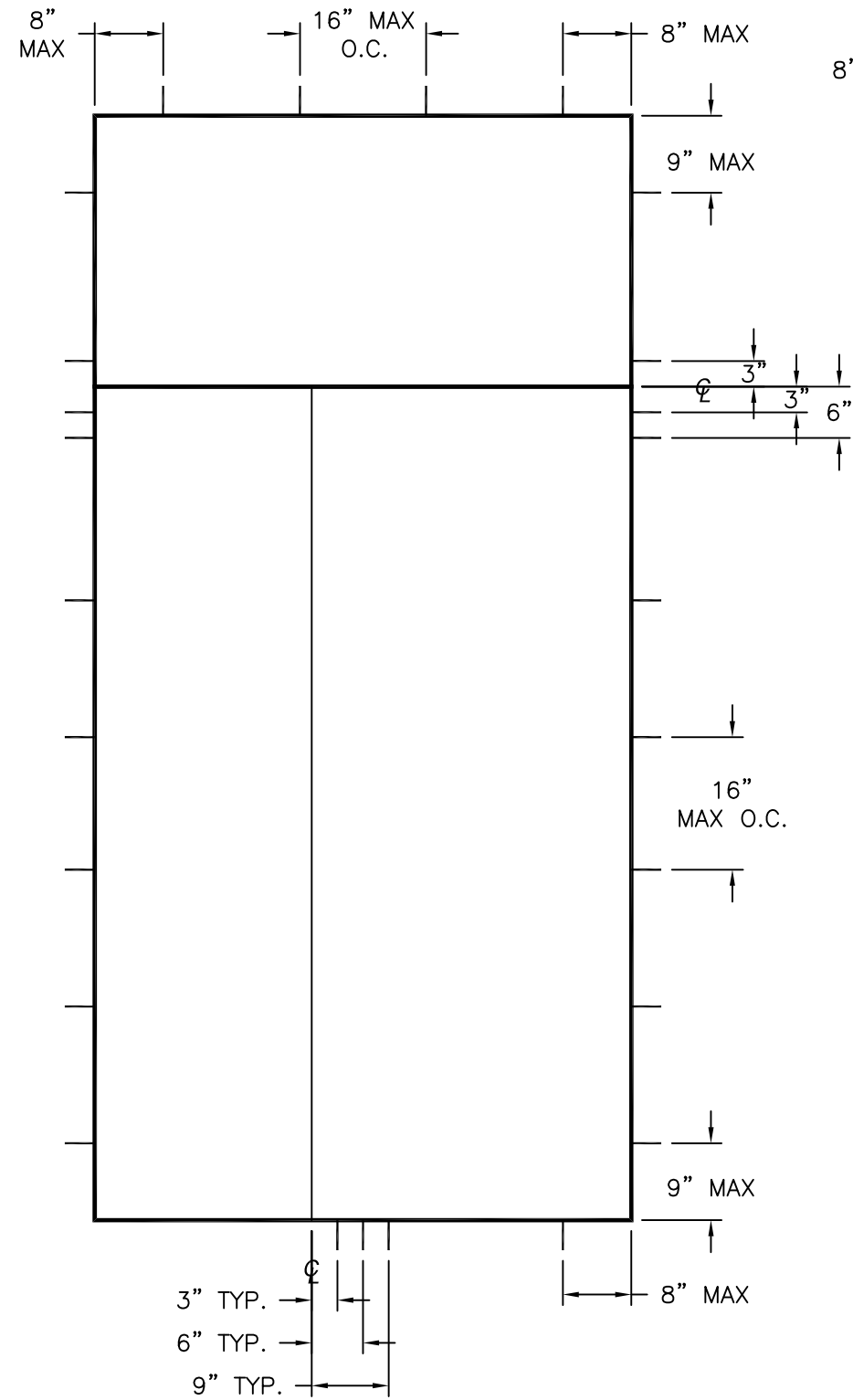
SINGLE W/SIDELITE AND TRANSOM
