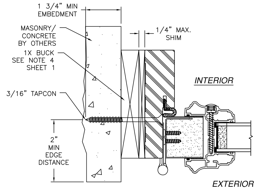
HORIZONTAL CROSS SECTION DOOR INSTALLATION CONCRETE/MASONRY
