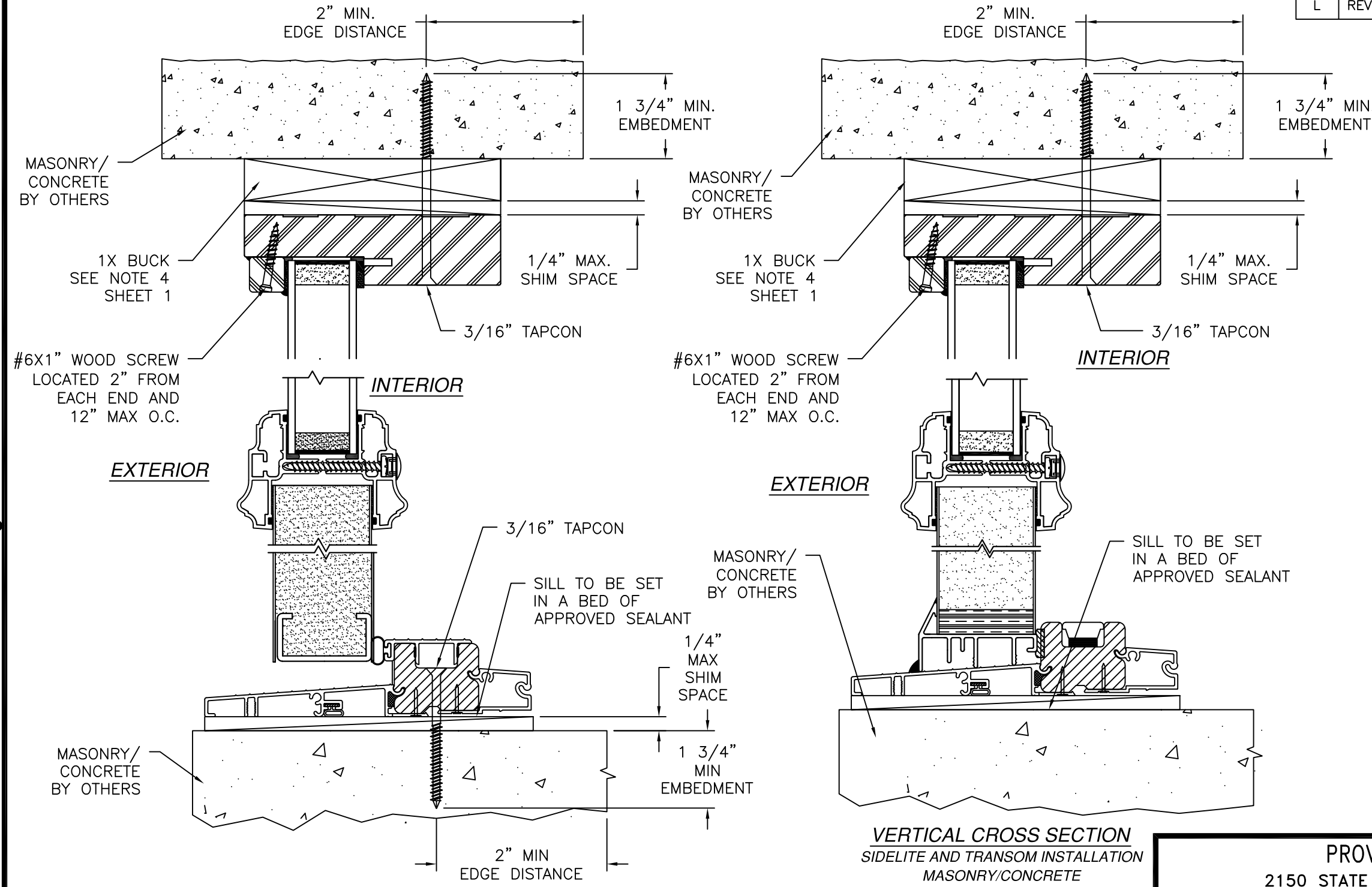
VERTICAL CROSS SECTION DOOR AND TRANSOM INSTALLATION MASONRY/CONCRETE TRANSOM HEAD SHOWN TRANSOM JAMB SIMILAR
