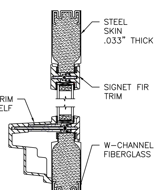
OPTION 12 SIGNET FIR & DENTIL SHELF TRIM
