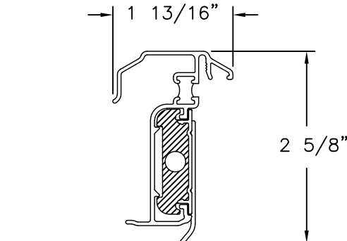
HURRICANE ASTRAGAL DETAIL
