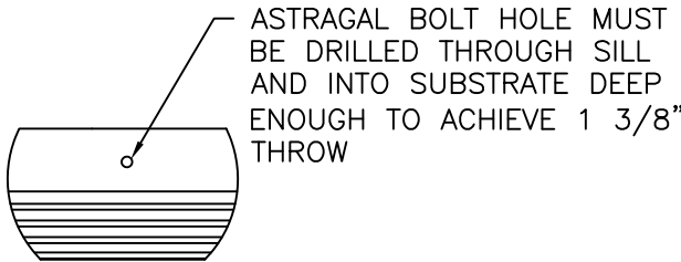
ASTRAGAL SILL DETAIL
