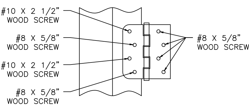
HINGE INSTALLATION DETAIL 2X BUCK/WOOD FRAMING
