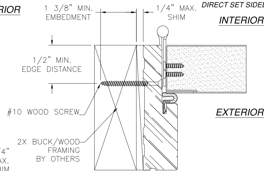
HORIZONTAL CROSS SECTION DOOR INSTALLATION - 2X BUCK/WOOD FRAMING SIGNED: 11/27/2023
