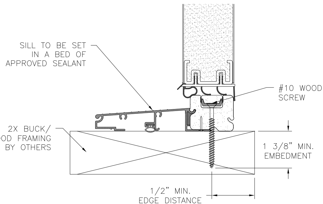
VERTICAL CROSS SECTION DOOR INSTALLATION - 2X BUCK/WOOD FRAMING
