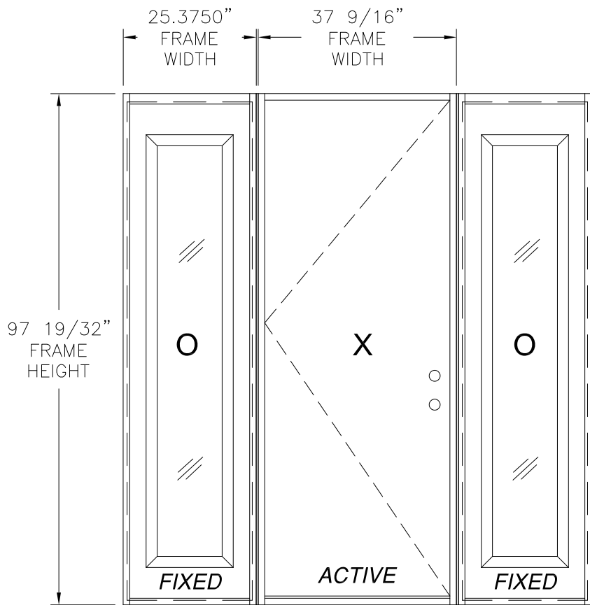
SINGLE W/ STD SIDELITES EXTERIOR VIEW
