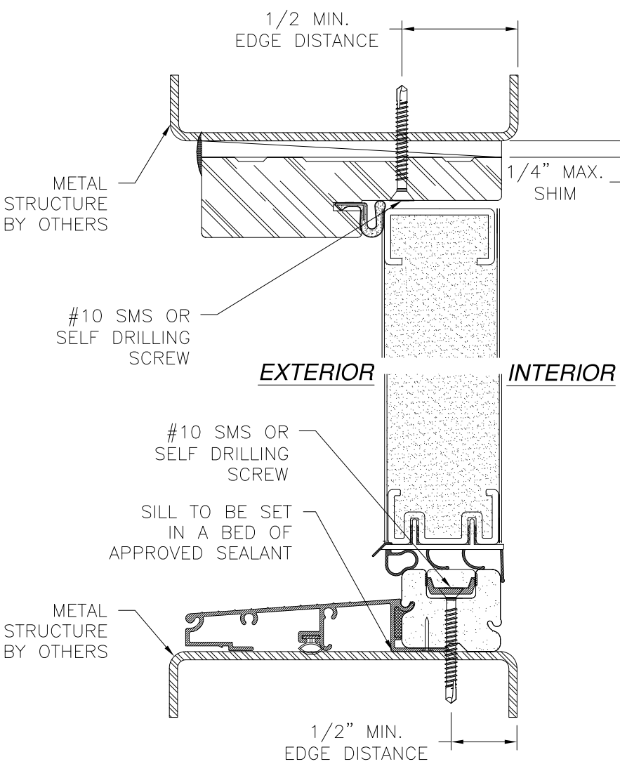
VERTICAL CROSS SECTION DOOR INSTALLATION METAL STRUCTURE
