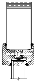
SIGNET TRIM
