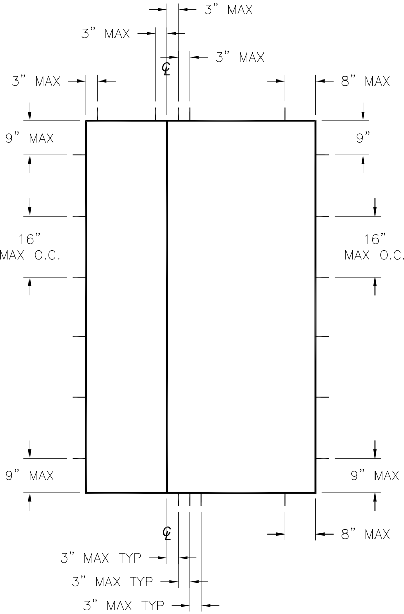
SINGLE W/SIDELITE
