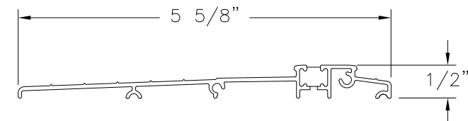
ADA THRESHOLD
