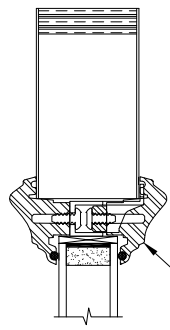
STANDARD TRIM
