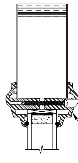
TRINITY TRIM
