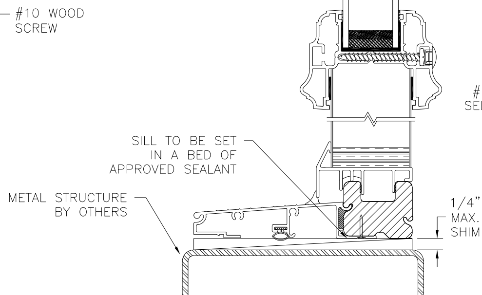
VERTICAL CROSS SECTION SIDELITE INSTALLATION 2X BUCK/WOOD FRAMING STANDARD SIDELITE SHOWN DIRECT SET SIDELITE SIMILAR
