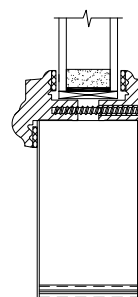
OPTION 14 XLE TRIM
