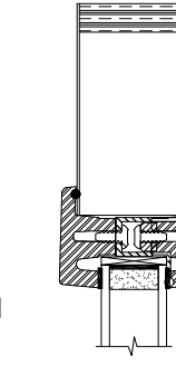
ELTON TRIM
