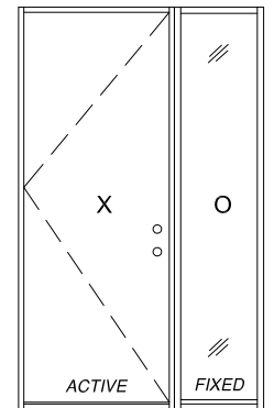
SINGLE W/ DIRECT SET SIDELITE EXTERIOR VIEW
