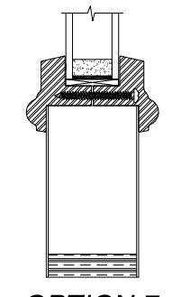
OPTION 7 RSL TRIM
