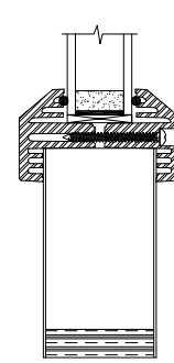
OPTION 6 SPOTLIGHT TRIM
