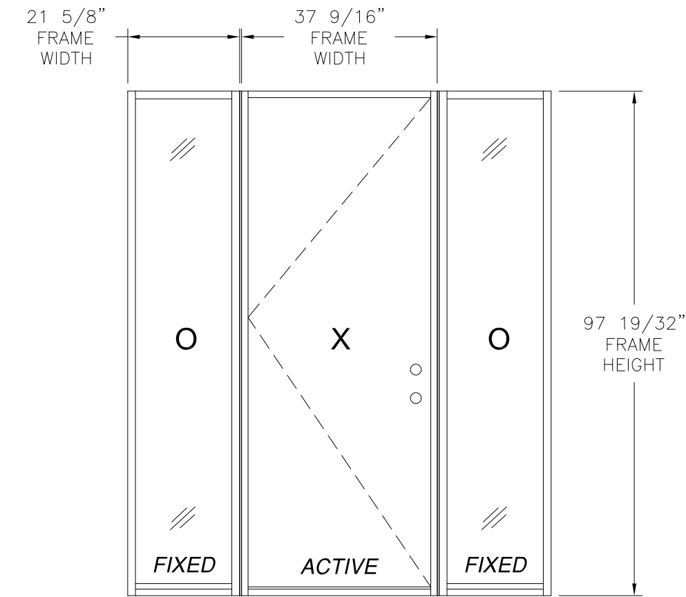
SINGLE W/ DIRECT SET SIDELITES EXTERIOR VIEW
