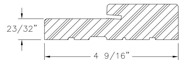
FRAMESAVER COMPOSITE
