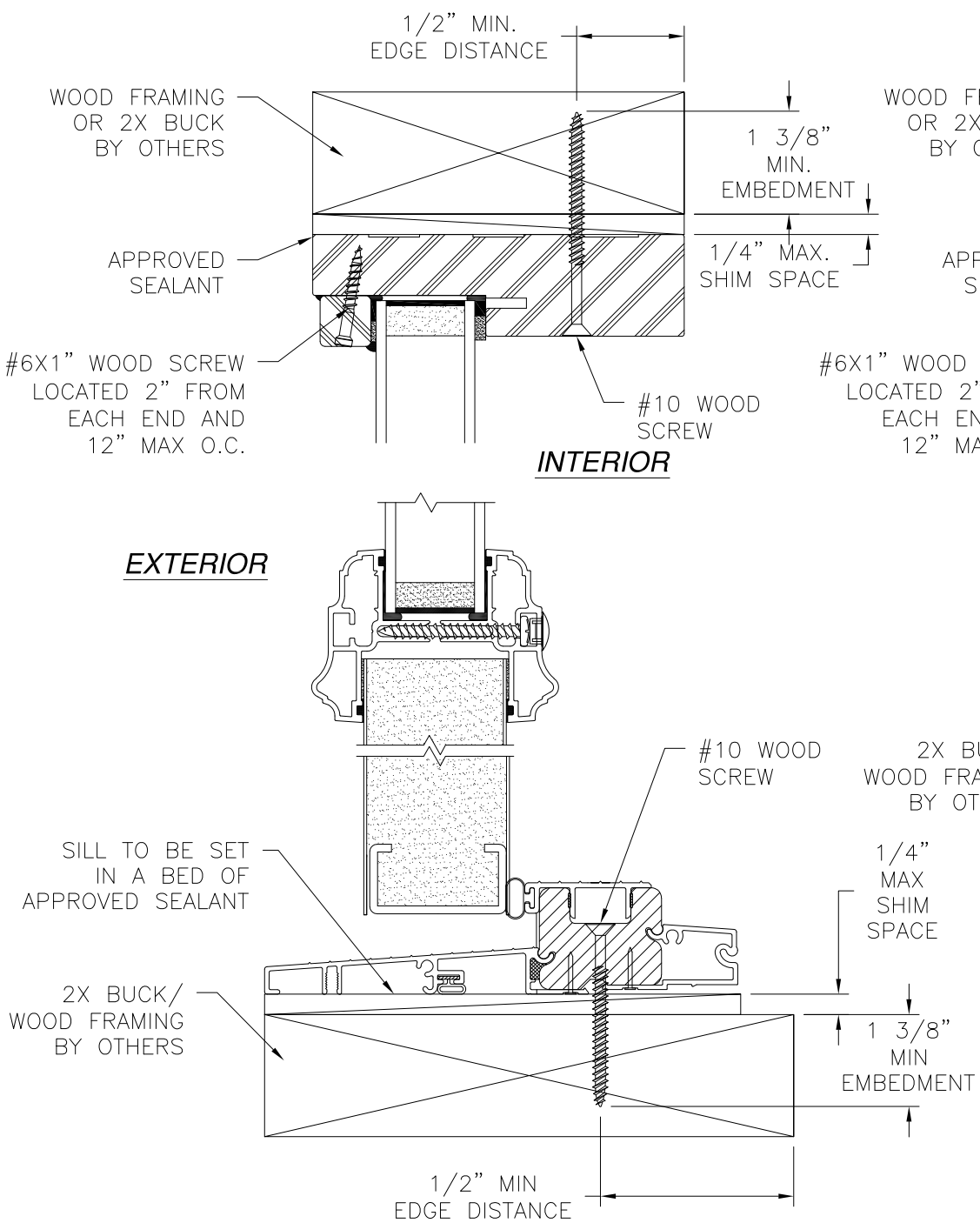
VERTICAL CROSS SECTION SIDELITE AND TRANSOM INSTALLATION 2X BUCK/WOOD FRAMING STANDARD SIDELITE SHOWN DIRECT SET SIDELITE SIMILAR TRANSOM HEAD SHOWN TRANSOM JAMB SIMILAR
