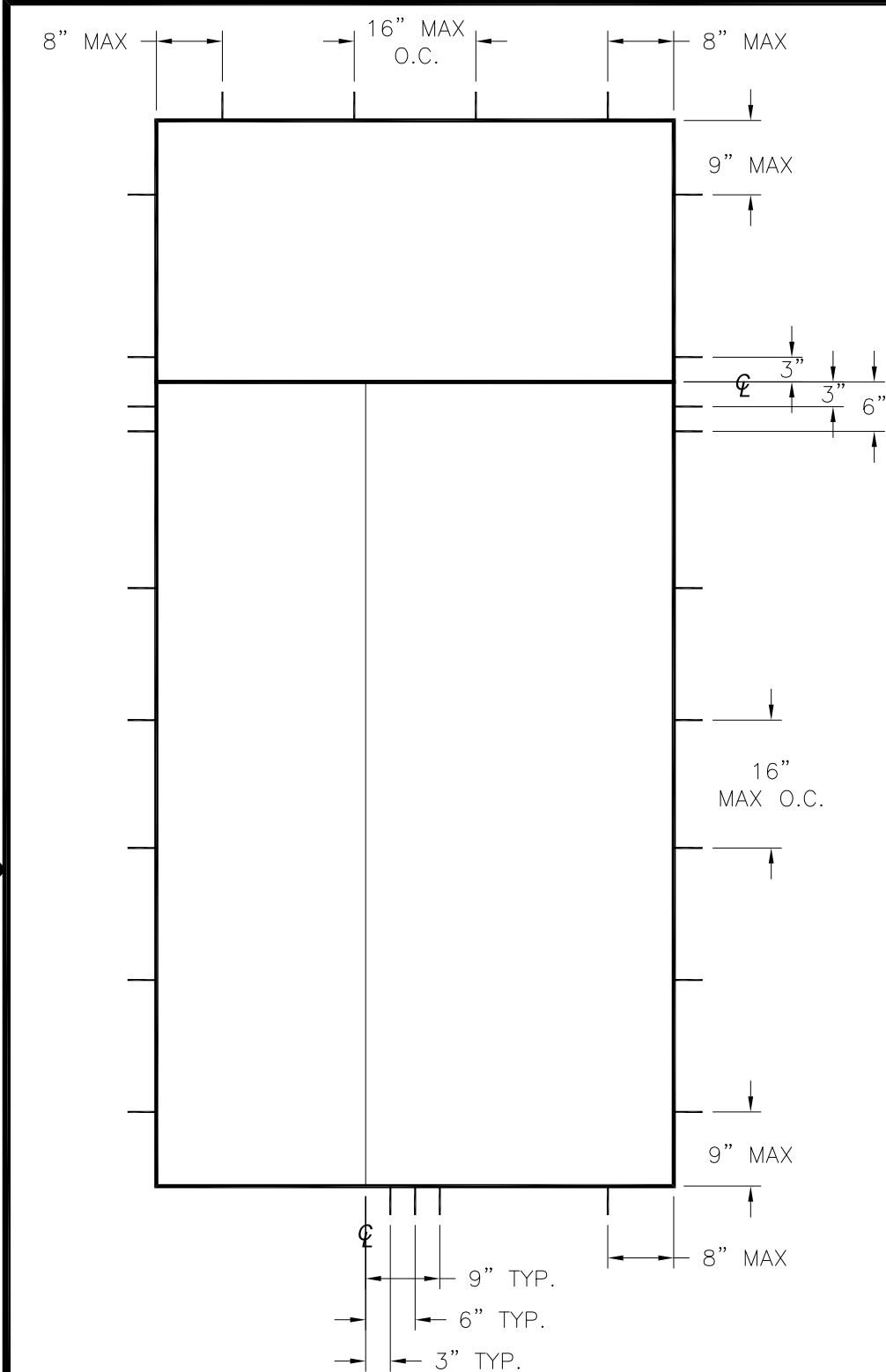
SINGLE W/SIDELITE AND TRANSOM
