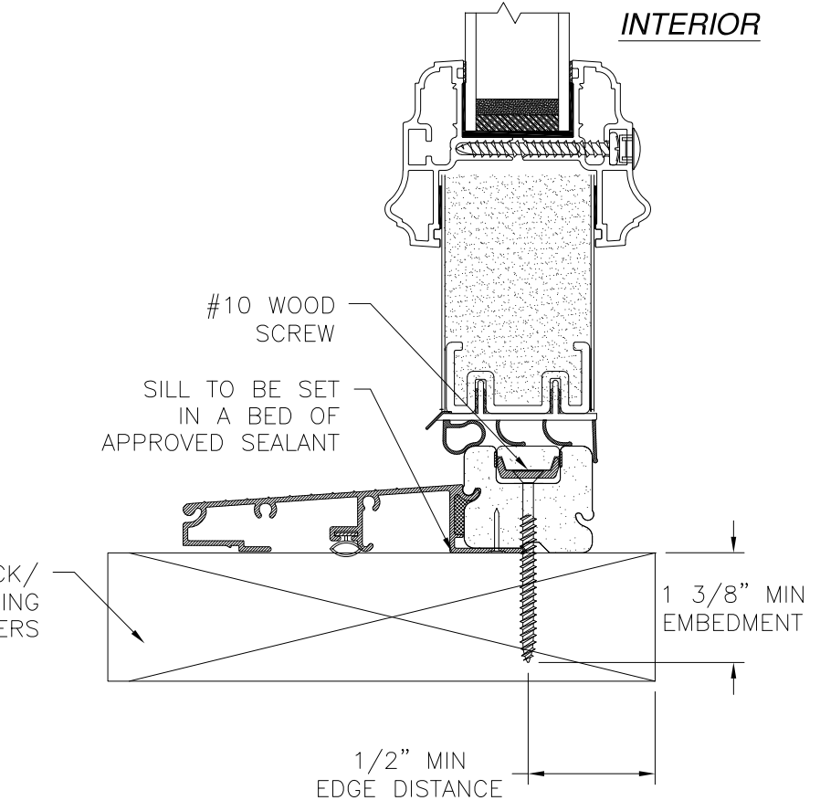
VERTICAL CROSS SECTION DOOR AND TRANSOM INSTALLATION - 2X BUCK/WOOD FRAMING TRANSOM HEAD SHOWN TRANSOM JAMB SIMILAR
