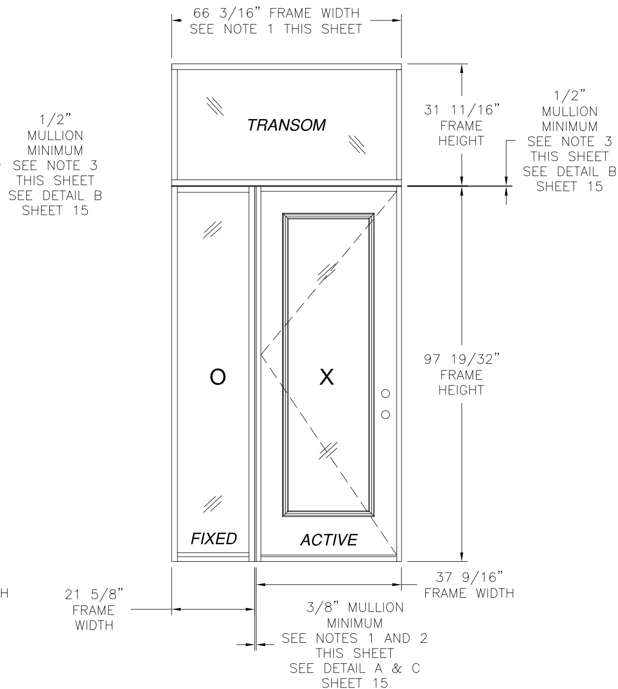
SINGLE W/ DIRECT SET SIDELITE AND TRANSOM EXTERIOR VIEW OX SHOWN XO ALSO APPROVED
